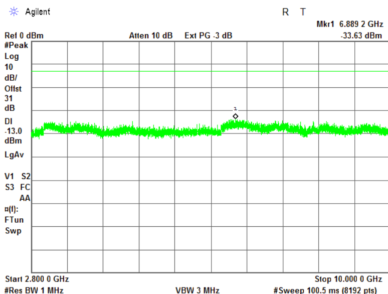
Plot 7.4.20 Spurious emission measurements in 2800 - 10000 MHz at mid carrier frequency
