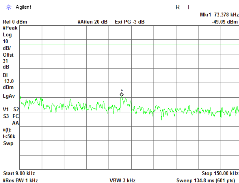
Plot 7.4.3 Spurious emission measurements in 9 - 150 kHz range at high carrier frequency
