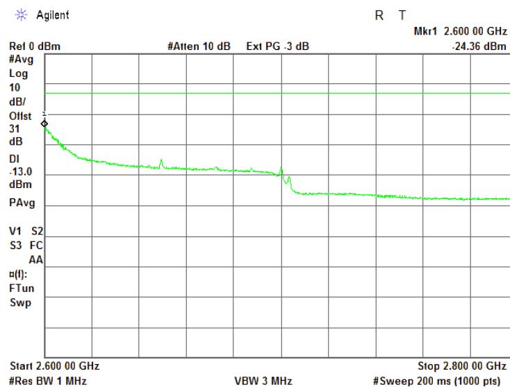
Plot 7.4.17 Spurious emission measurements in 2600 - 2800 MHz at mid carrier frequency
