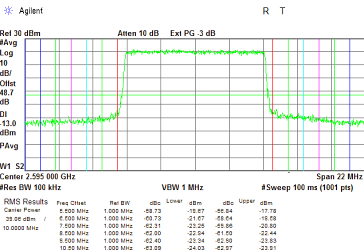
Plot 7.3.12 Spurious emission at band edges test results at high carrier frequency, 10 MHz EBW
