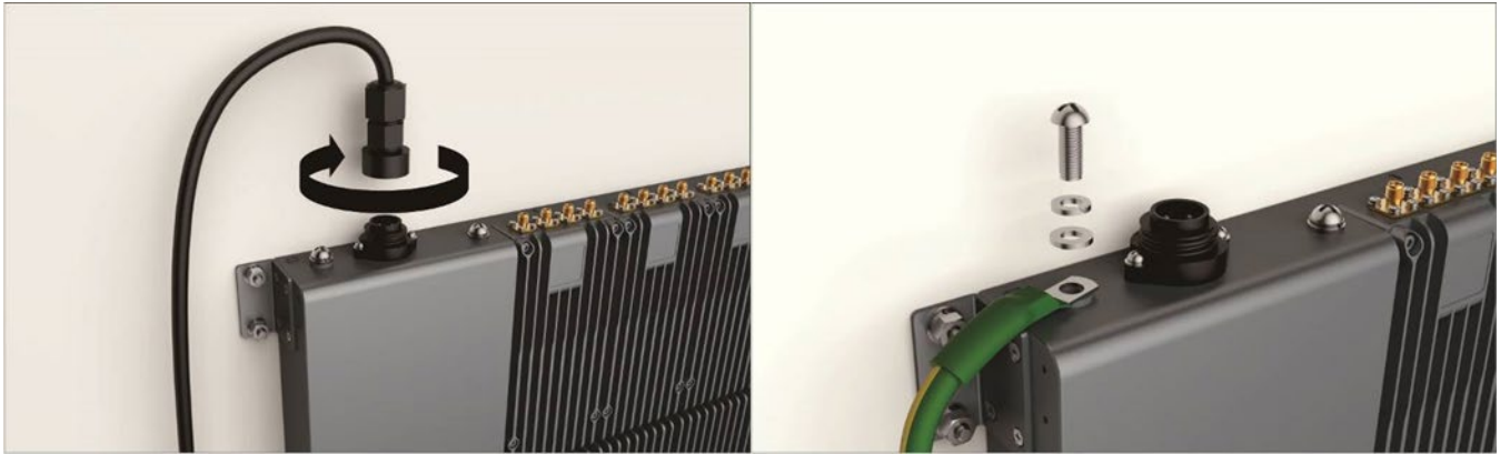
Figure 12. Connect Power and Ground Cables
