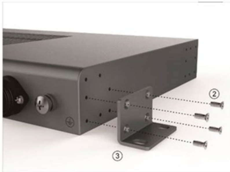
Figure 22. Attach Handles
