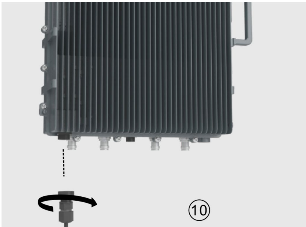
Figure 46. Connect the Power Cable of E62-X3
