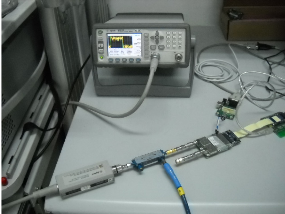
Photograph No.1 Peak output power measurement setup
