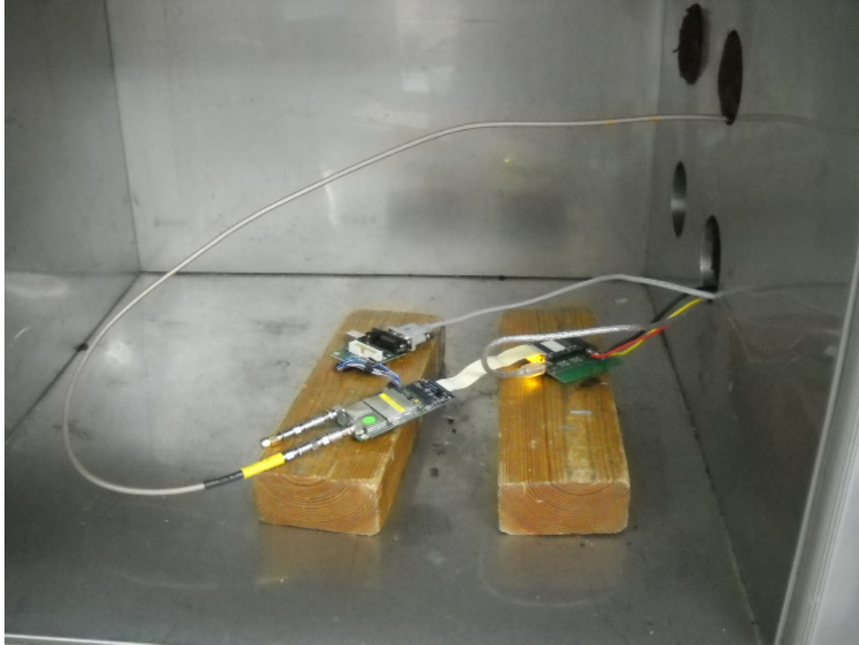
Photograph No.8 Frequency stability measurement setup
