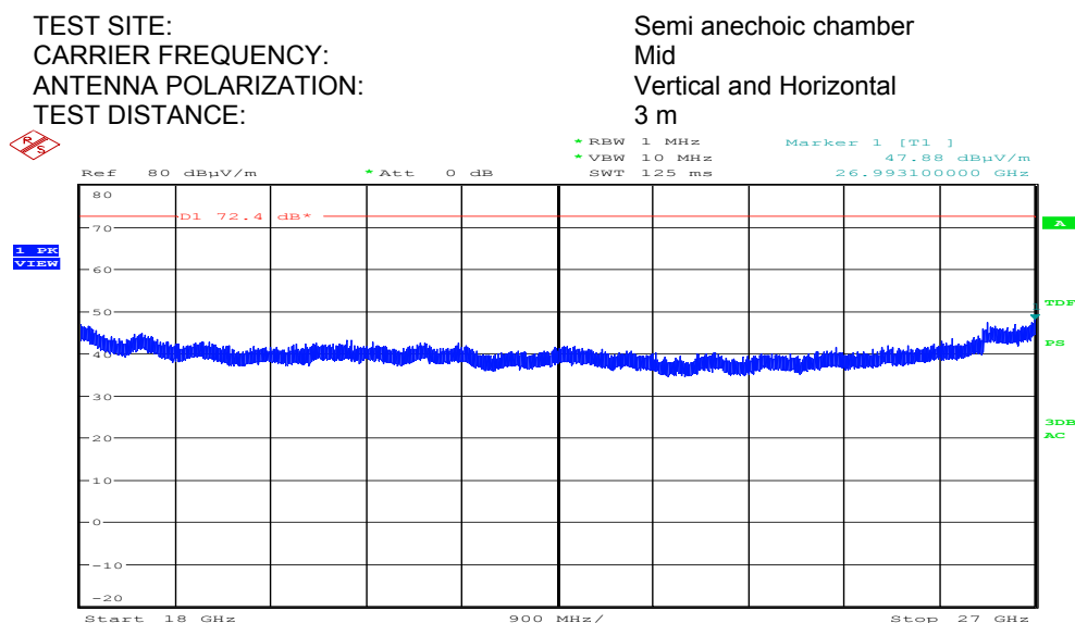
Plot 7.5.17 Radiated emission measurements in 18000 – 27000 MHz range
