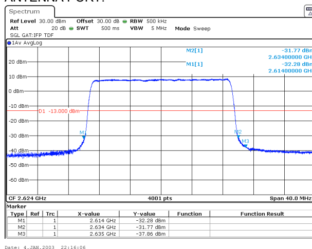
Plot 7.3.33 Spurious emission at band edges test results at high carrier frequency
