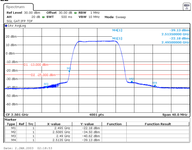
Plot 7.3.20 Spurious emission at band edges test results at mid carrier frequency
