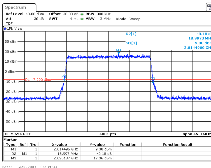
Plot 7.1.14 Occupied bandwidth test result at mid frequency, 20 MHz EBW, 16QAM, RF chain #22
