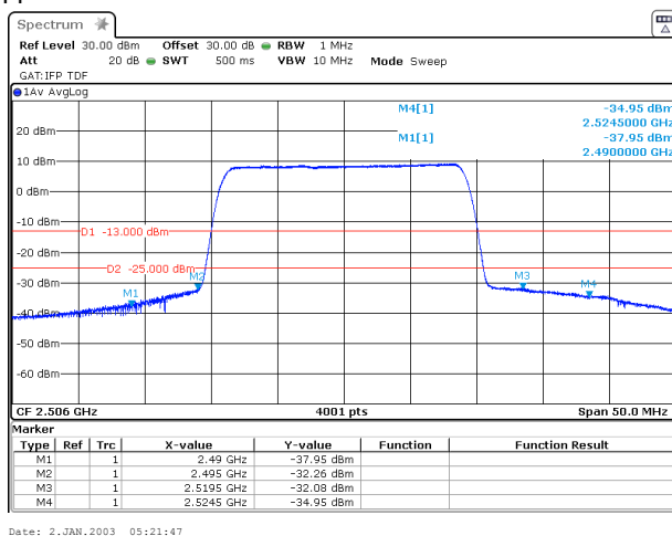
Plot 7.3.11 Spurious emission at band edges test results at mid carrier frequency
