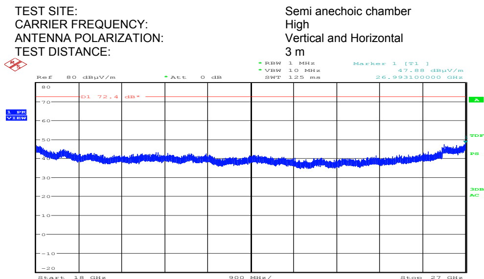
Plot 7.5.18 Radiated emission measurements in 18000 – 27000 MHz range
