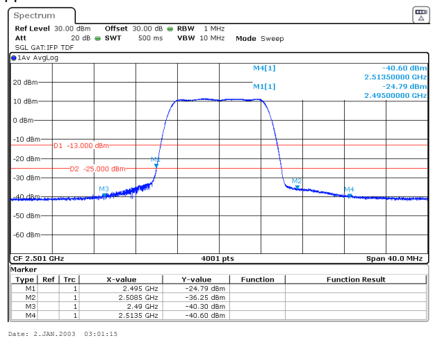
Plot 7.3.8 Spurious emission at band edges test results at mid carrier frequency
