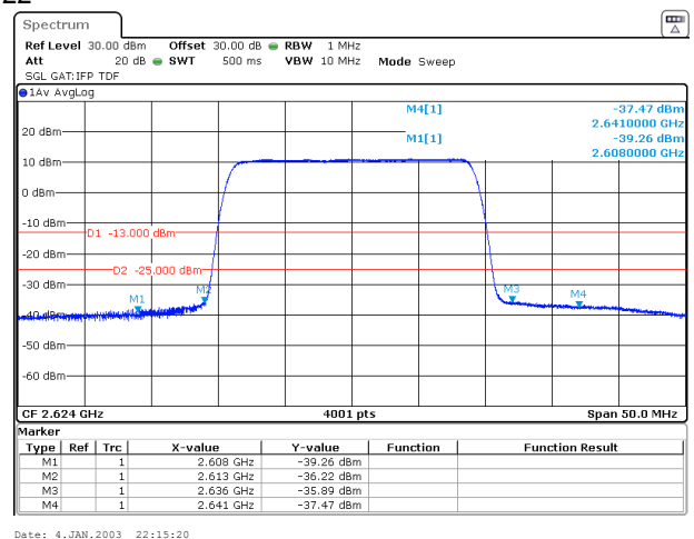
Plot 7.3.33 Spurious emission at band edges test results at high carrier frequency
