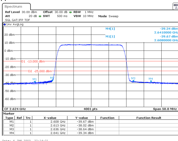
Plot 7.3.15 Spurious emission at band edges test results at high carrier frequency
