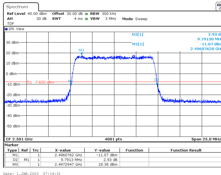
Plot 7.1.26 Occupied bandwidth test result at mid frequency, 10 MHz EBW, 64QAM, RF chain #12
