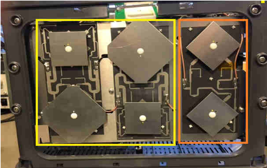
Backhaul Antenna
