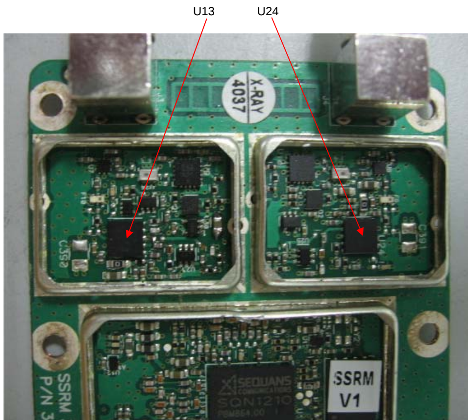
Photograph No.3 SSRM 3.65GHz module without shielding close view
