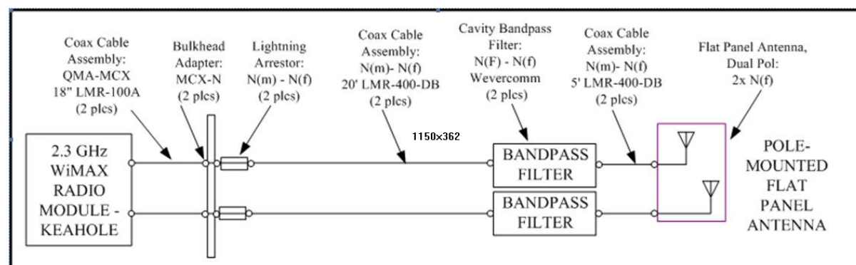
Figure 1 - Block Diagram
