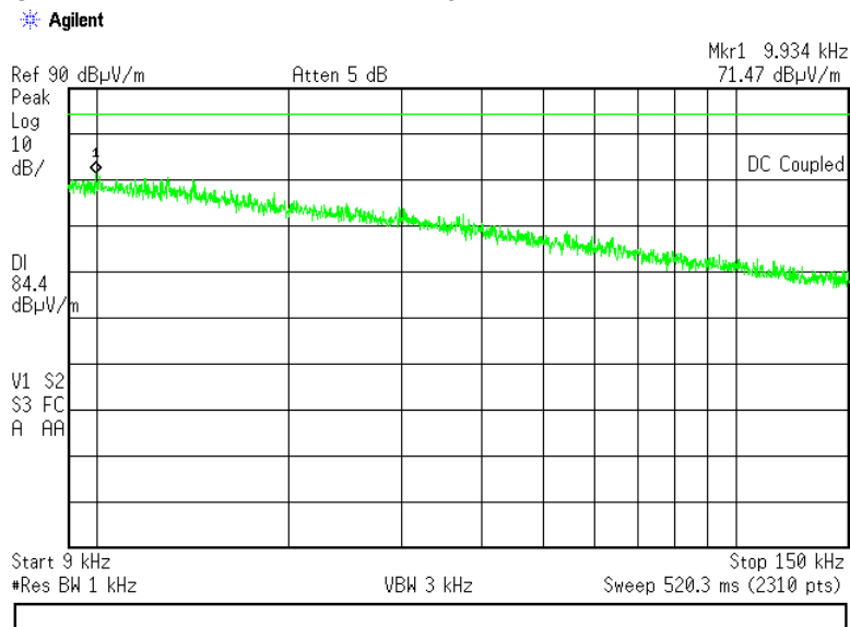
Plot 7.4.2 Radiated emission measurements in 9 - 150 kHz range
