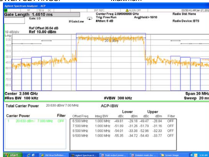
Plot 7.3.18 Emission mask test results at high carrier frequency, 10 MHz EBW
