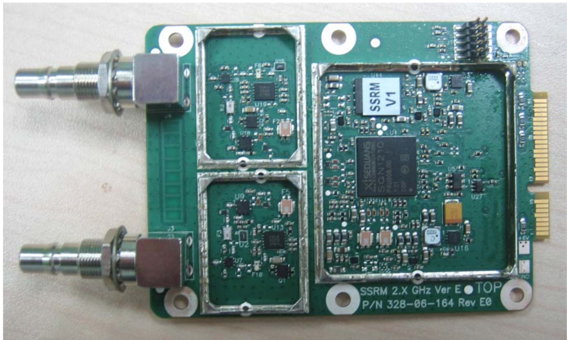
Photograph No.1 SSRM 2.5 GHz module without shielding
