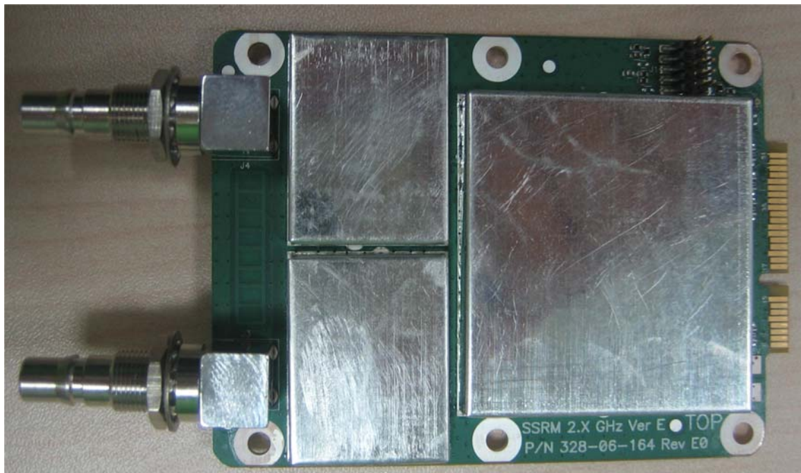
Photograph No.1 SSRM 2.3 GHz module top view
