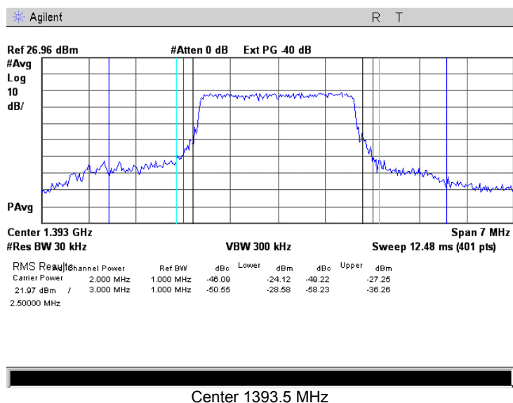
Plot 7.4.55 Spurious emission measurements in 1390 – 1391 MHz, 1391 – 1392 MHz, 1395 – 1396 MHz, 1396 – 1397 MHz at mid carrier frequency, 2.5 MHz EBW, BPSK modulation
