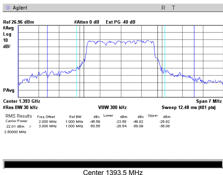
Plot 7.4.56 Spurious emission measurements in 1390 – 1391 MHz, 1391 – 1392 MHz, 1395 – 1396 MHz, 1396 - 1397 MHz at mid carrier frequency, 2.5 MHz EBW, 64QAM modulation
