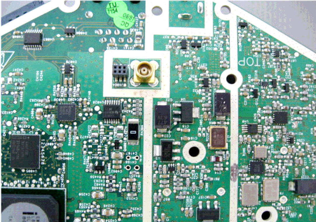
Photograph No.7 Main PCB second side close view
