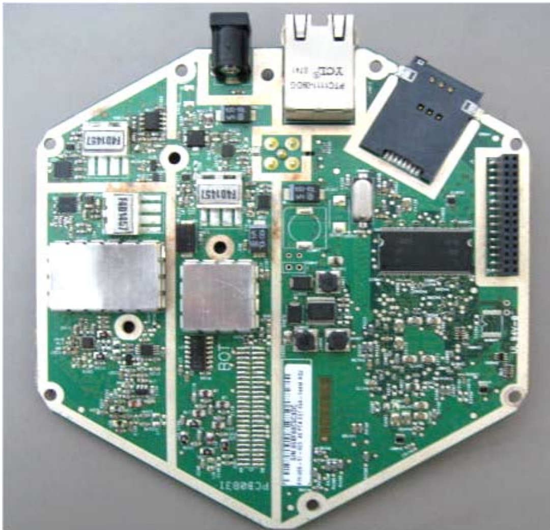
Photograph No.4 "ProST 1.4G TDD V-p" main PCB front view
