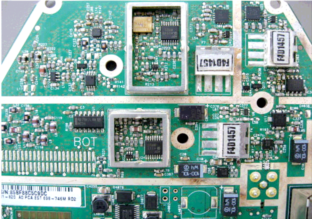
Photograph No.6 Main PCB front view without shields
