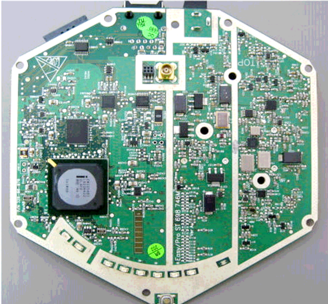
Photograph No.5 "ProST 1.4G TDD V-p" main PCB second side view
