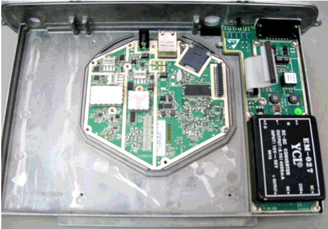
Photograph No.3 "ProST 1.4G TDD V-p" internal view with case removed
