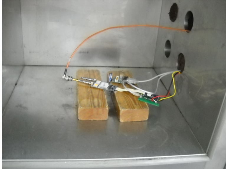
Photograph No.8 Frequency stability measurement setup
