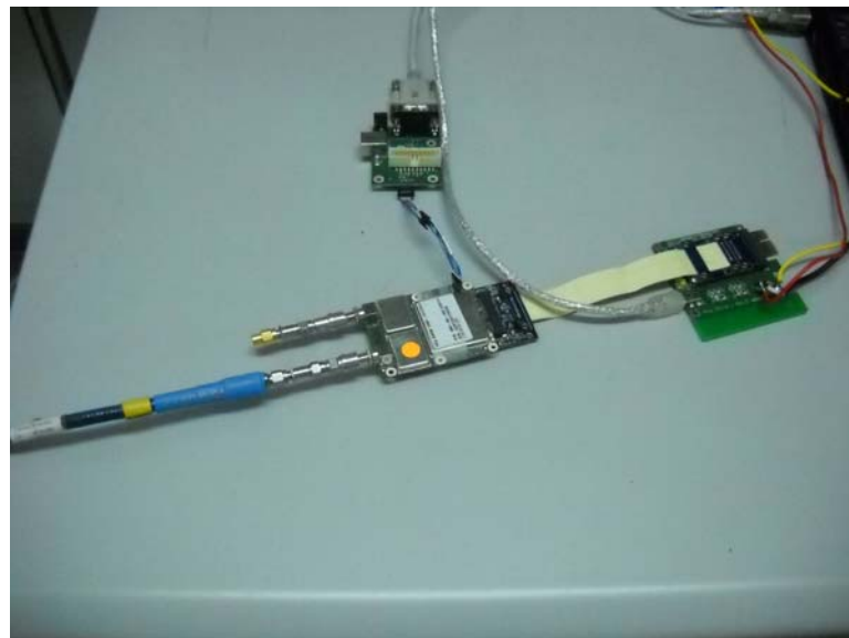
Photograph No.4 Occupied bandwidth and conducted spurious emissions measurement setup, EUT close view
