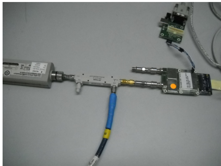
Photograph No.2 Peak output power measurement setup, EUT close view
