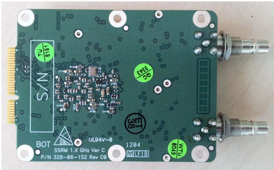
Photograph No.2 SSRM 1.4 GHz module bottom view
