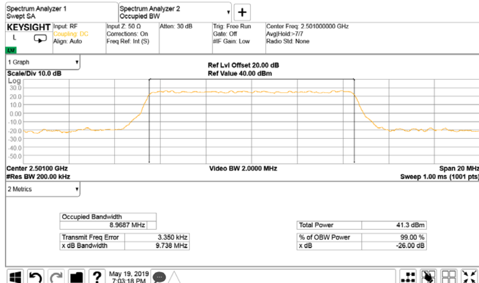
Plot 7.1.4 Occupied bandwidth test results at low frequency, 10 MHz EBW, 64QAM
