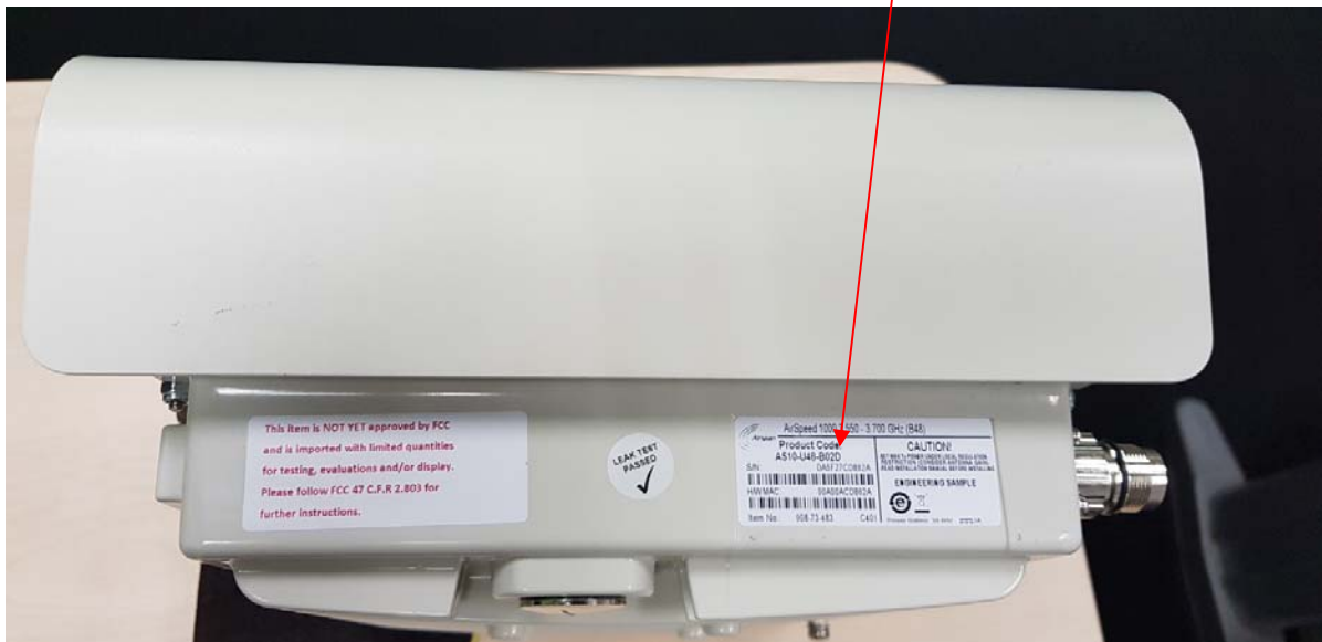
“AirSpeed 1000 3.550-3.700 GHz (B48)” side panel, label with FCC ID:PIDAS1000 location
