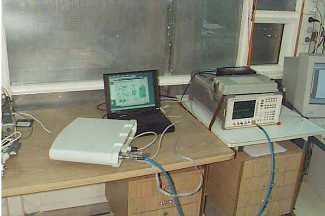
Photograph No.6 Conducted spurious emissions measurement setup
