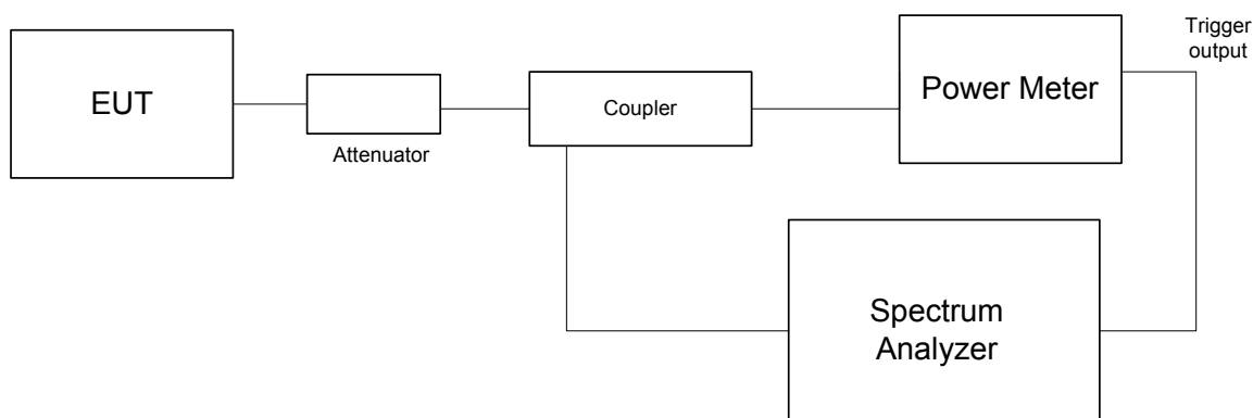
Figure 7.2.1 Peak output power test setup
