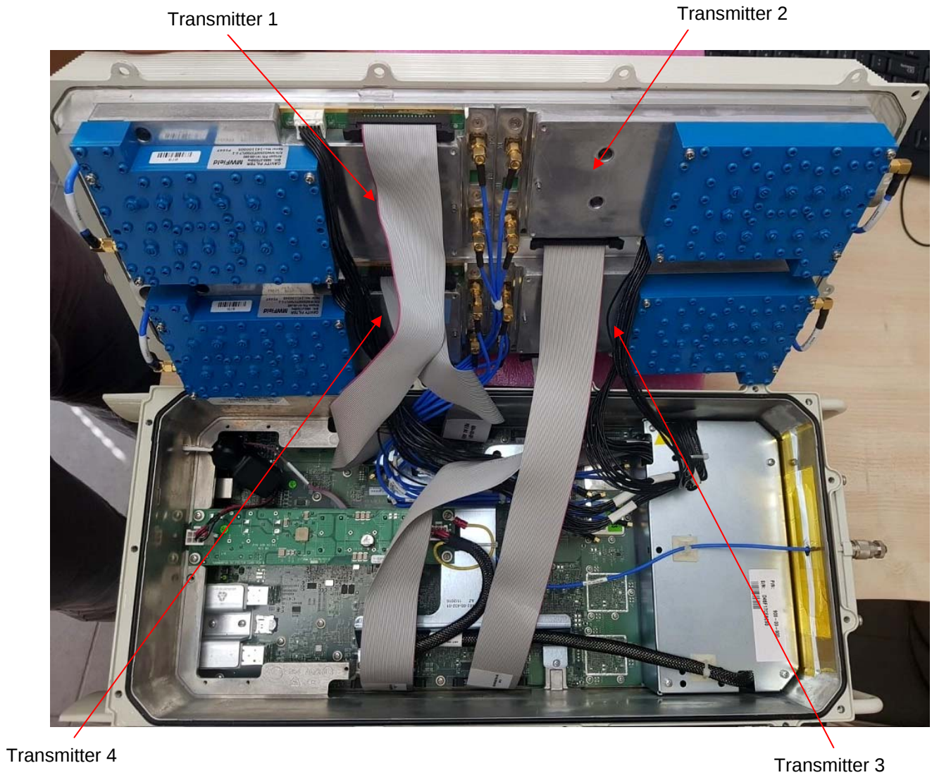
Photograph No.1 “AirHarmony 4200” base station internal view
