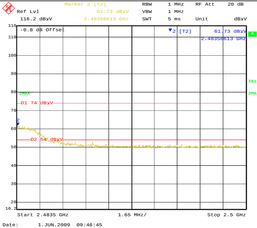
High Channel –Horizontal-Peak (802.11g)
