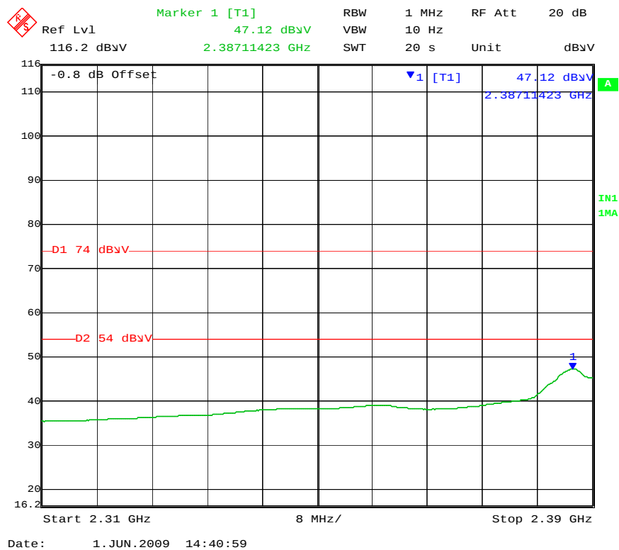
Low Channel –Vertical-Average (802.11b)
