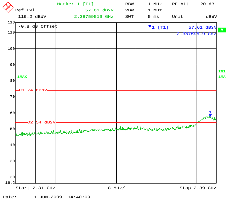
Low Channel –Vertical-Peak (802.11b)
