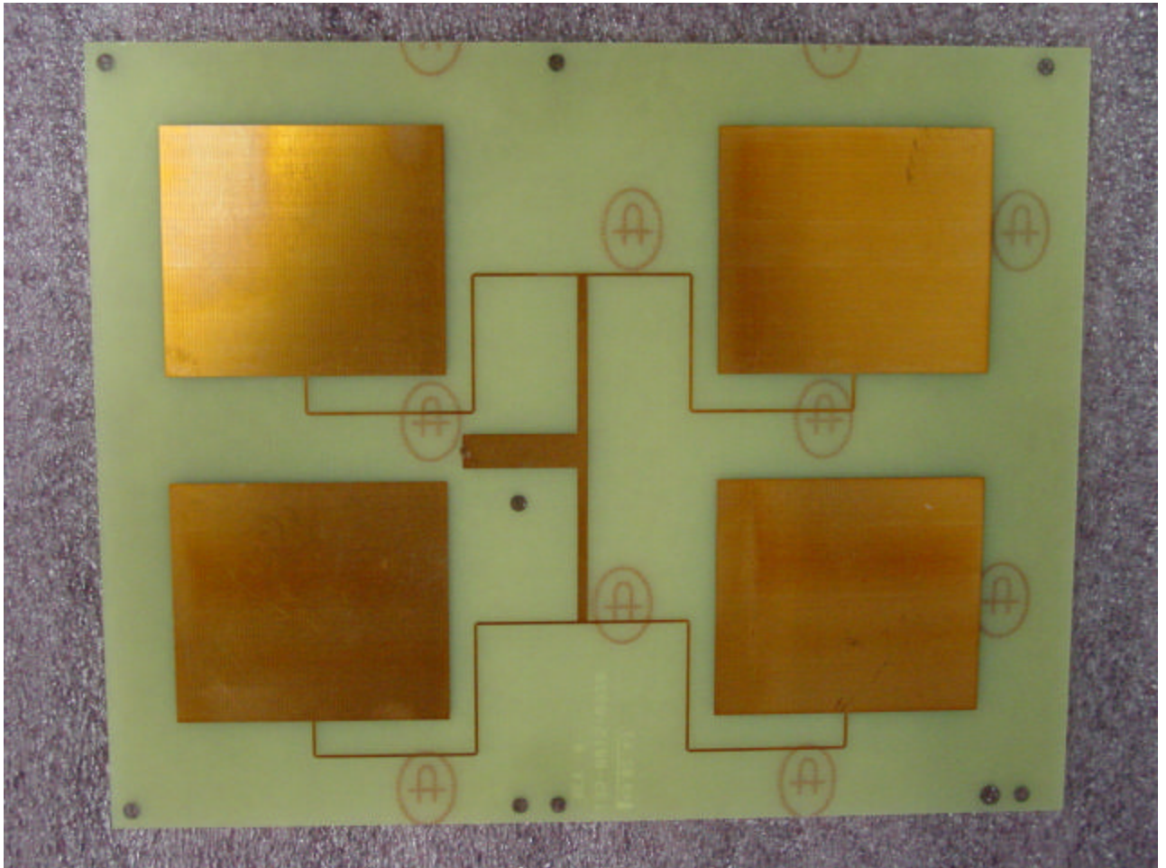
Horizontally Polarized Antenna (copper side)
