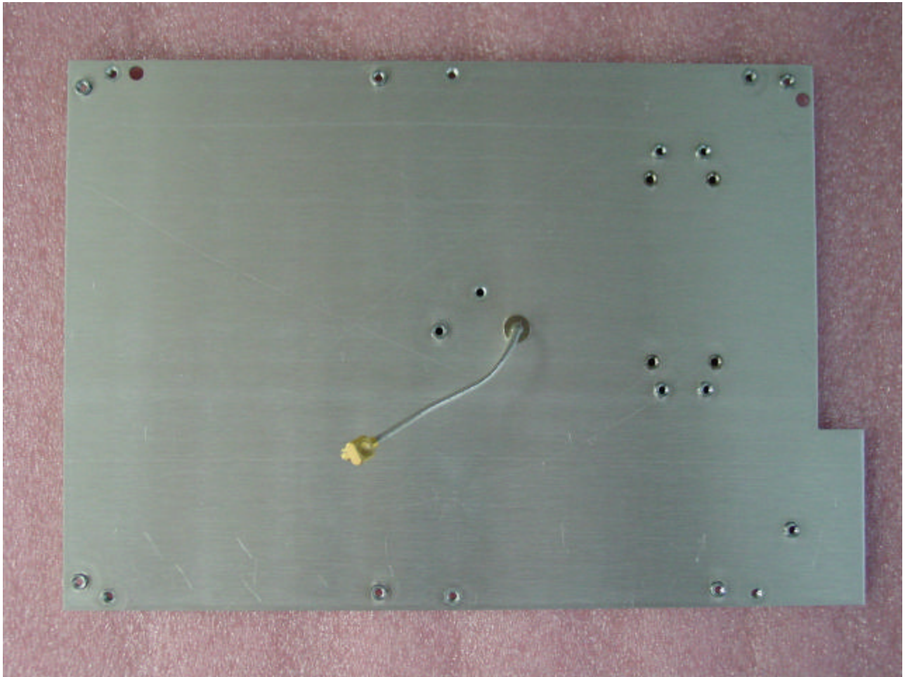
Antenna Plate (back side)
