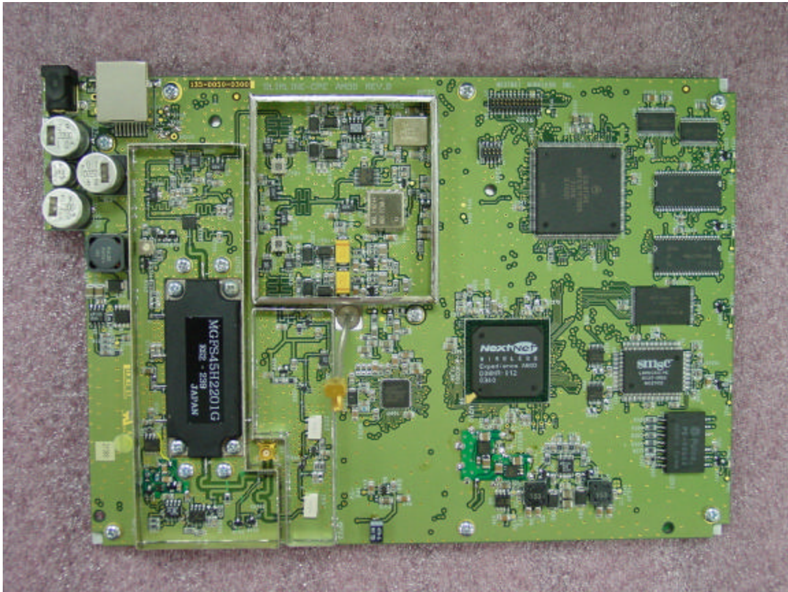
RF Board component side (no shields)
