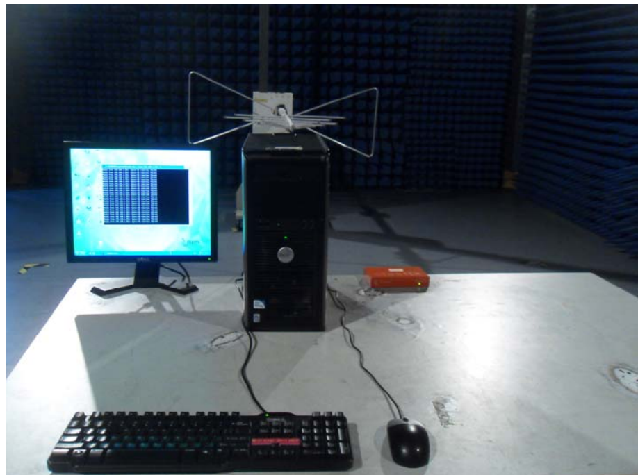
2.Photo of Radiated Emission Test
