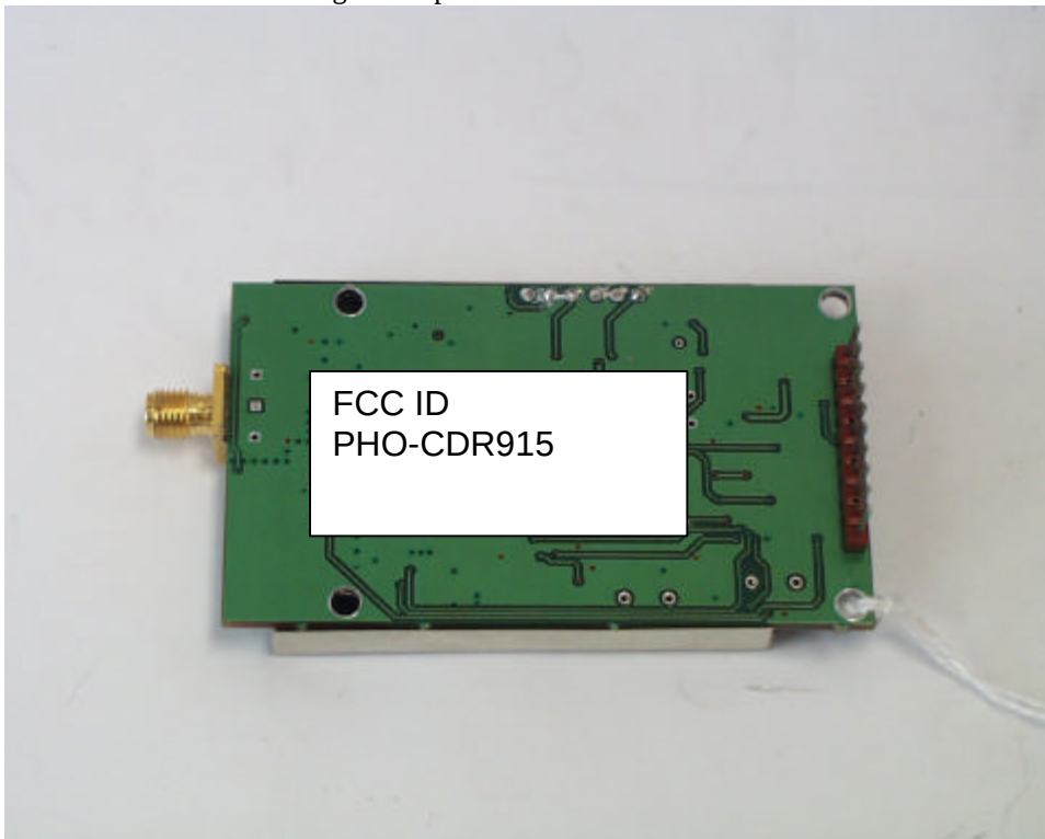
Bottom side of PCB showing solder plane and label.
