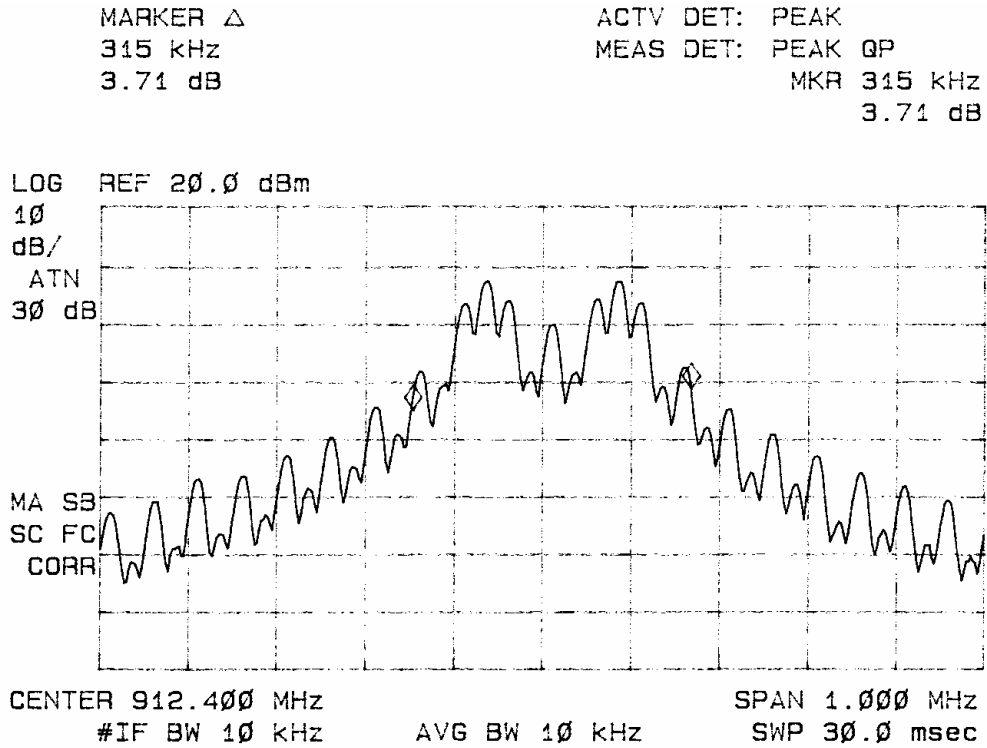
Figure 9. 20-dB bandwidth.
