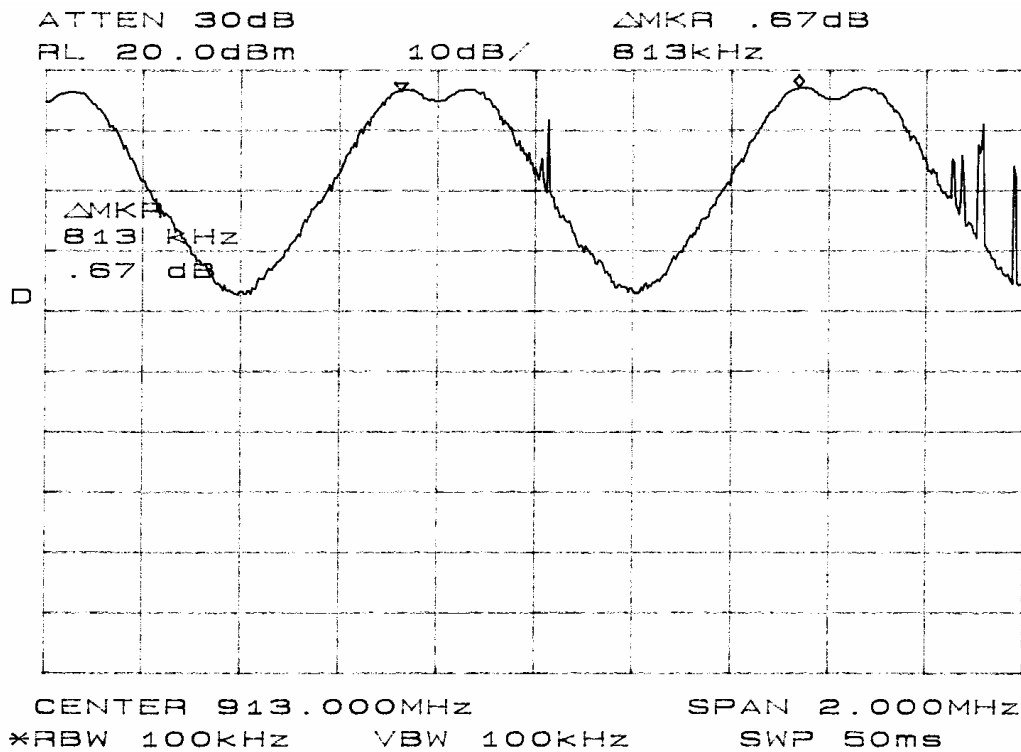
Figure 10 Channel Spacing.
