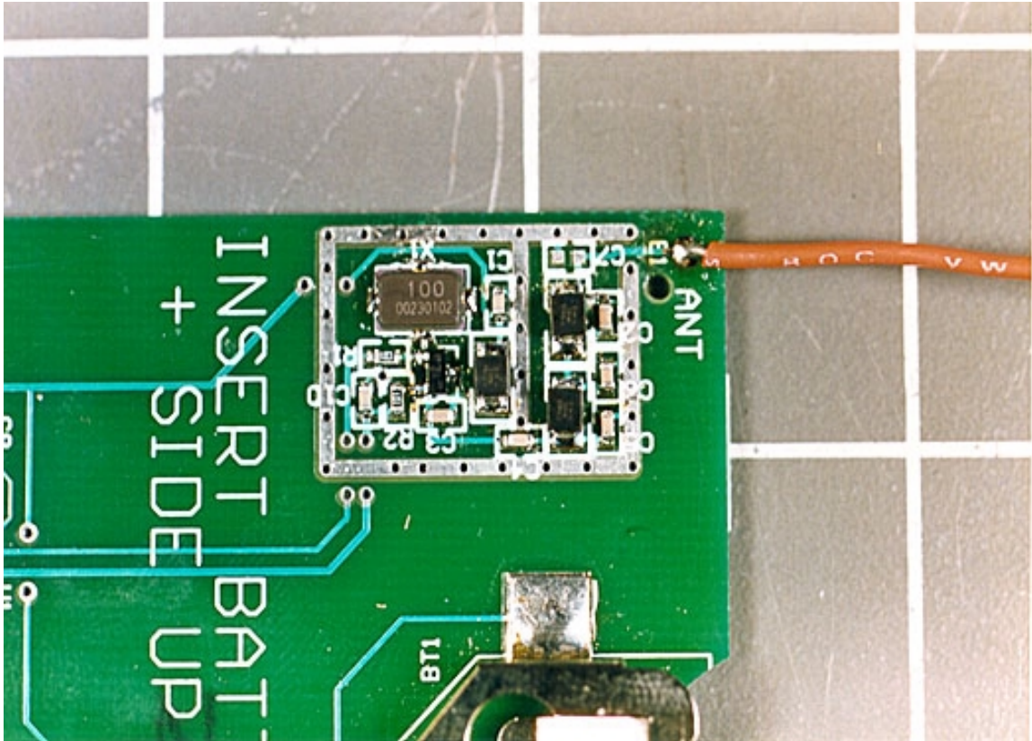
Close-up of Transmitter Circuitry
