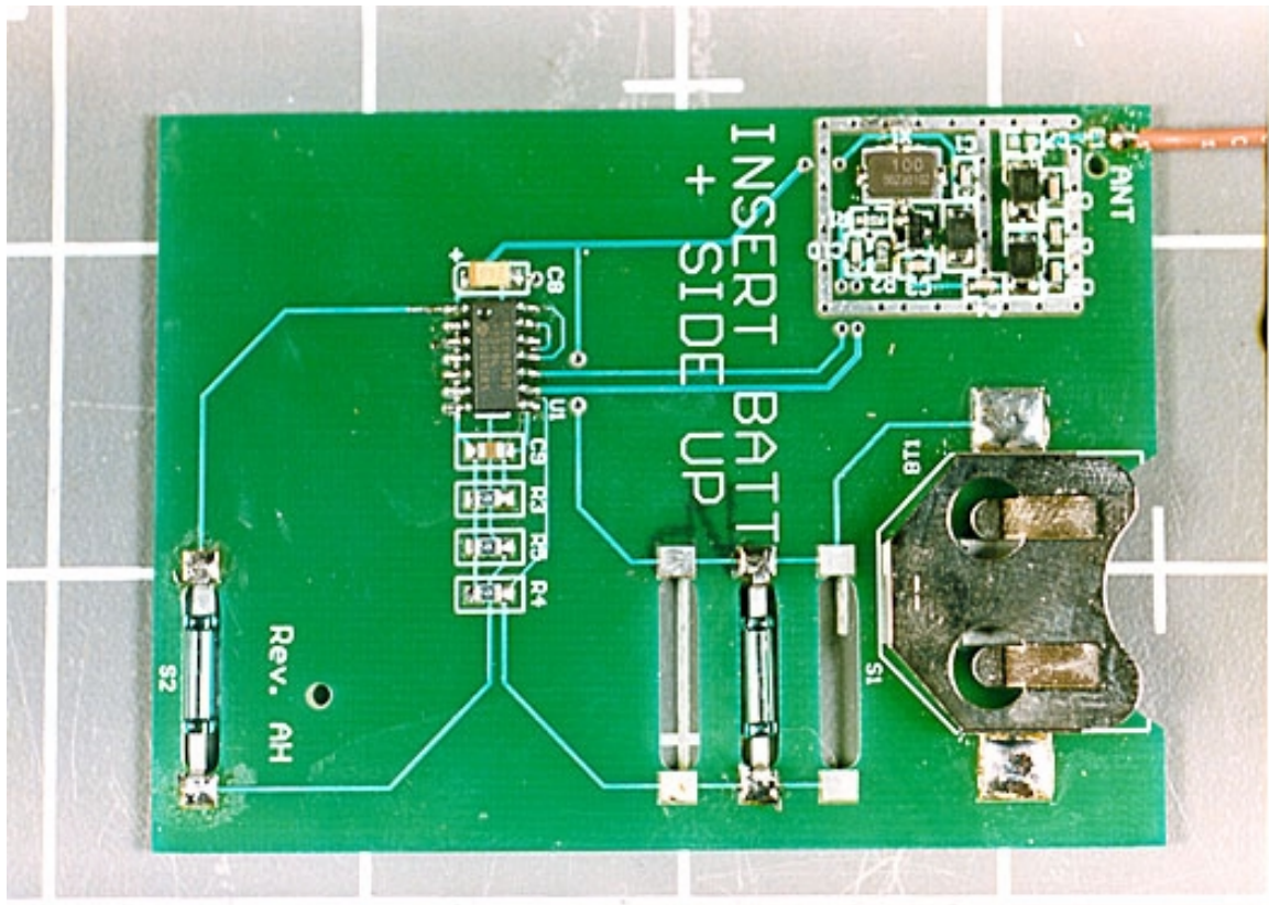
Back of PCB without Shield
