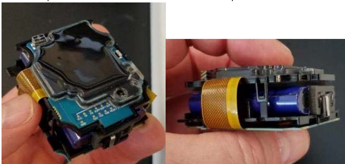
Encapsulated Ventis Pro 4 and Ventis Pro 5 Wi-fi Battery Pack Board Assemblies
