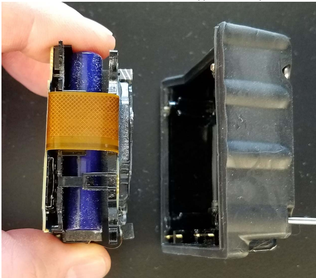
Ventis Pro 4 and Ventis Pro 5 Wi-fi battery pack disassembly
