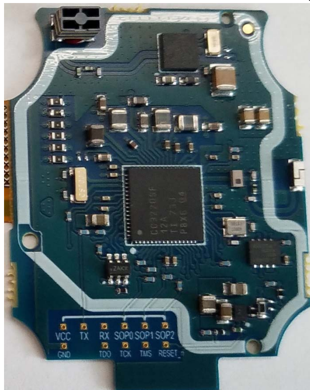
Ventis Pro 4 and Ventis Pro 5 Wi-fi Battery Board Top Component Side and Bottom Side
