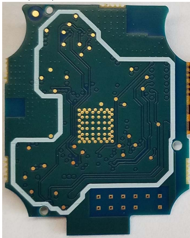
Ventis Pro 4 and Ventis Pro 5 Wi-fi Battery Board Top Component Side and Bottom Side
