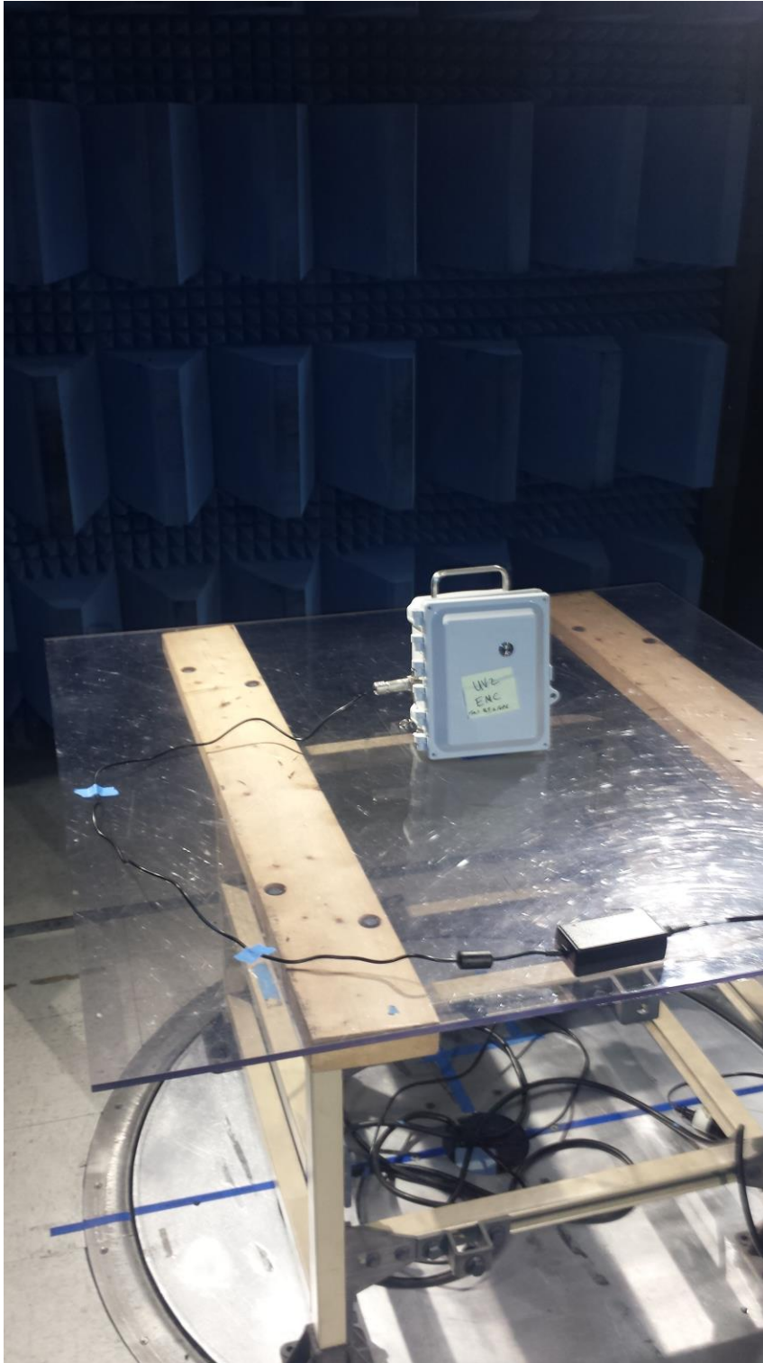
Placement of UUT and power supply in relation to ground plane.
