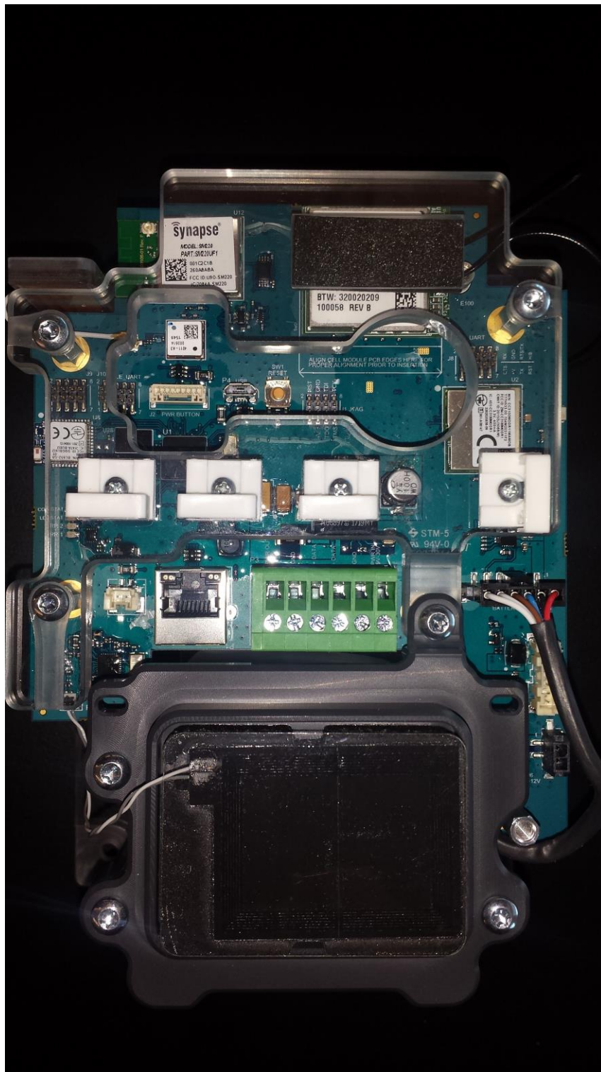
Carrier Front
