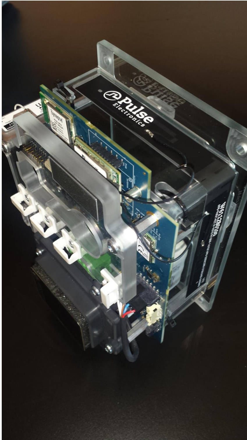
Carrier Right
