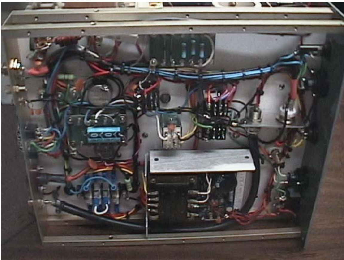
PLA-800 INTERNAL BOTTOM VIEW
