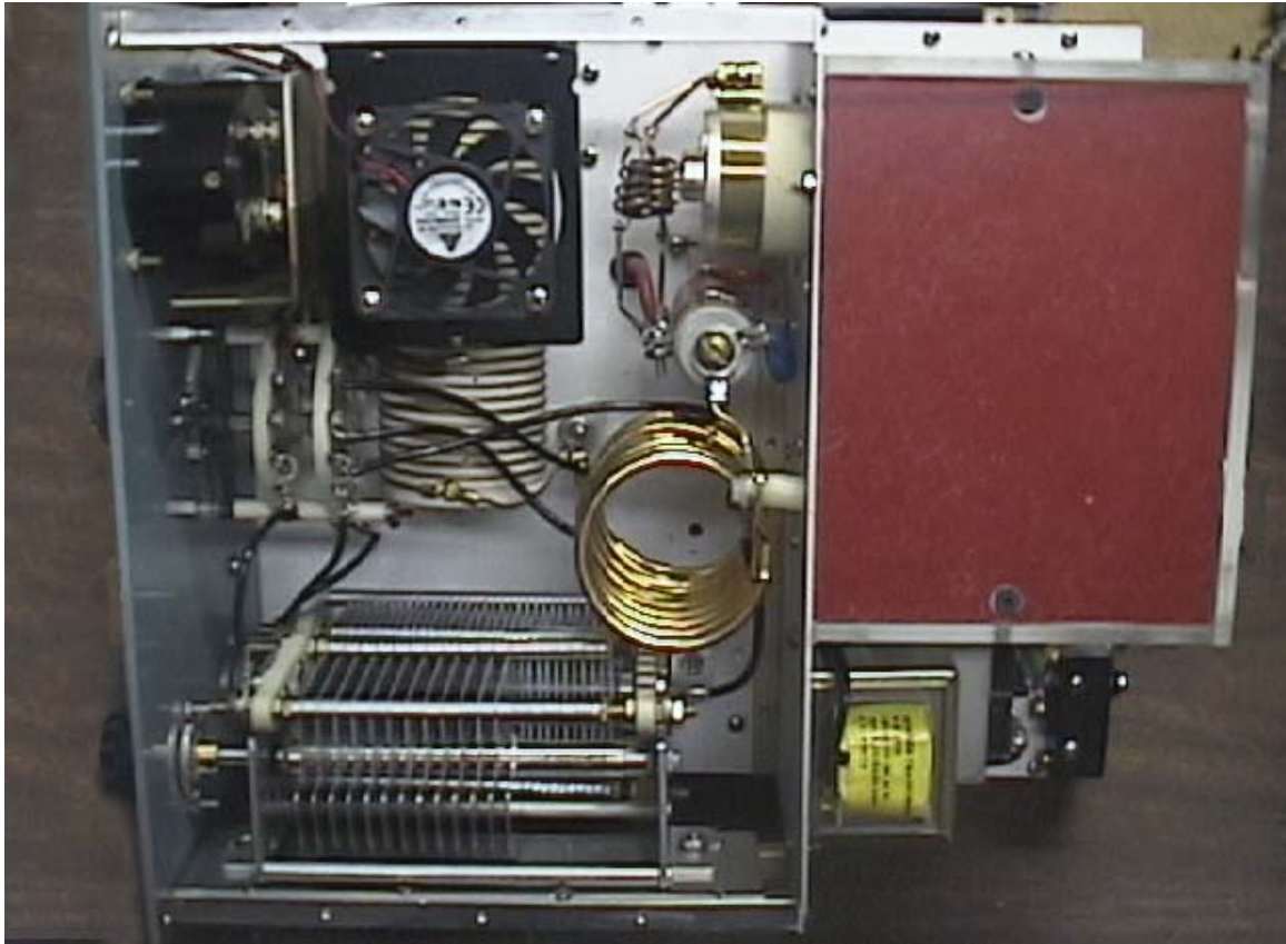
PLA-800 INTERNAL TOP VIEW
