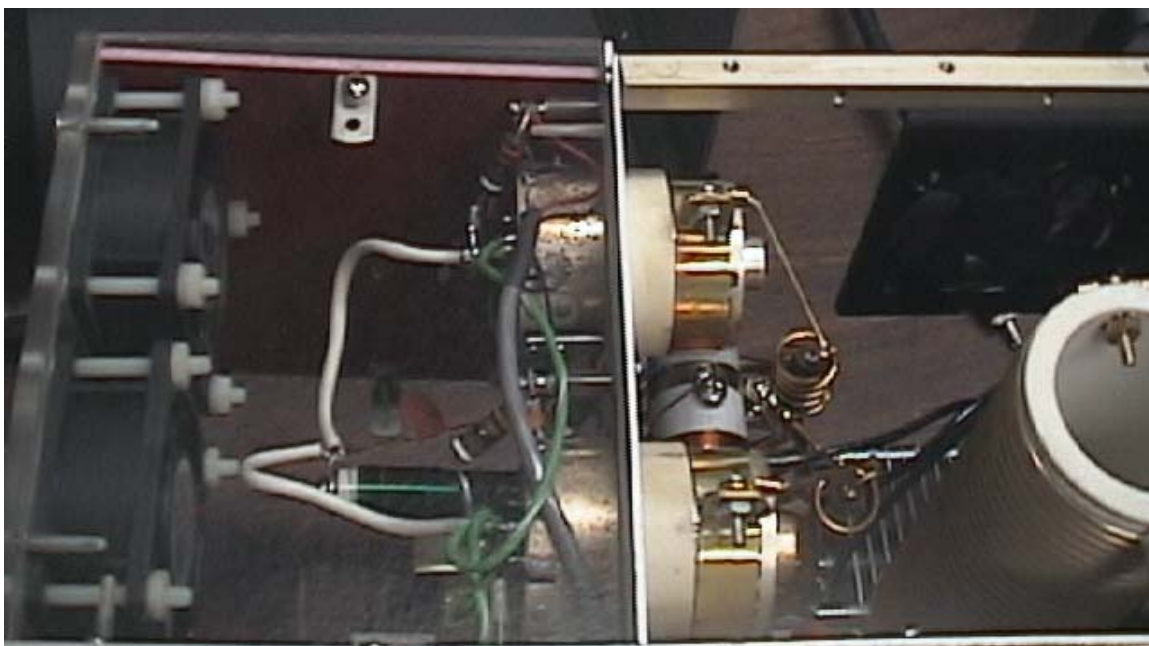
PLA-800 INTERNAL GRID CAGE
