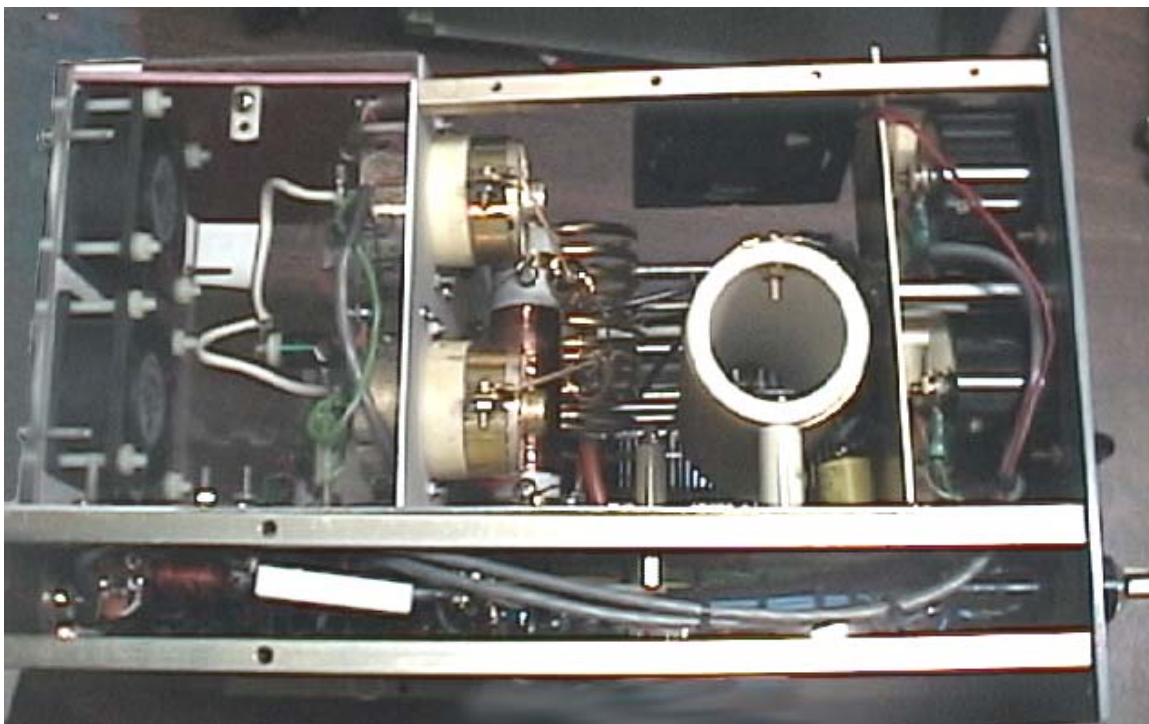
PLA-800 INTERNAL LEFT SIDE VIEW
