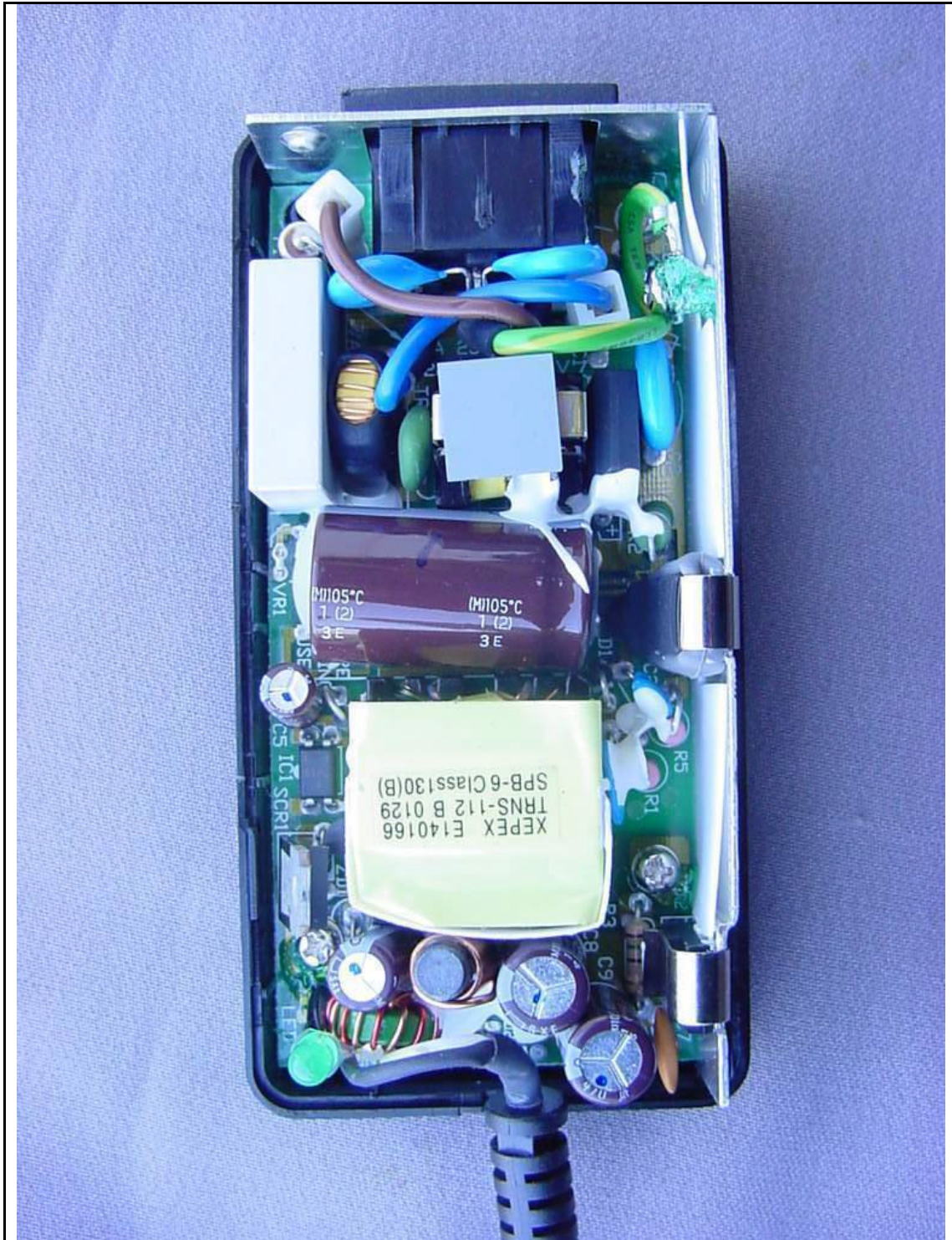
[ Top View of the AC/DC Adaptor ]
