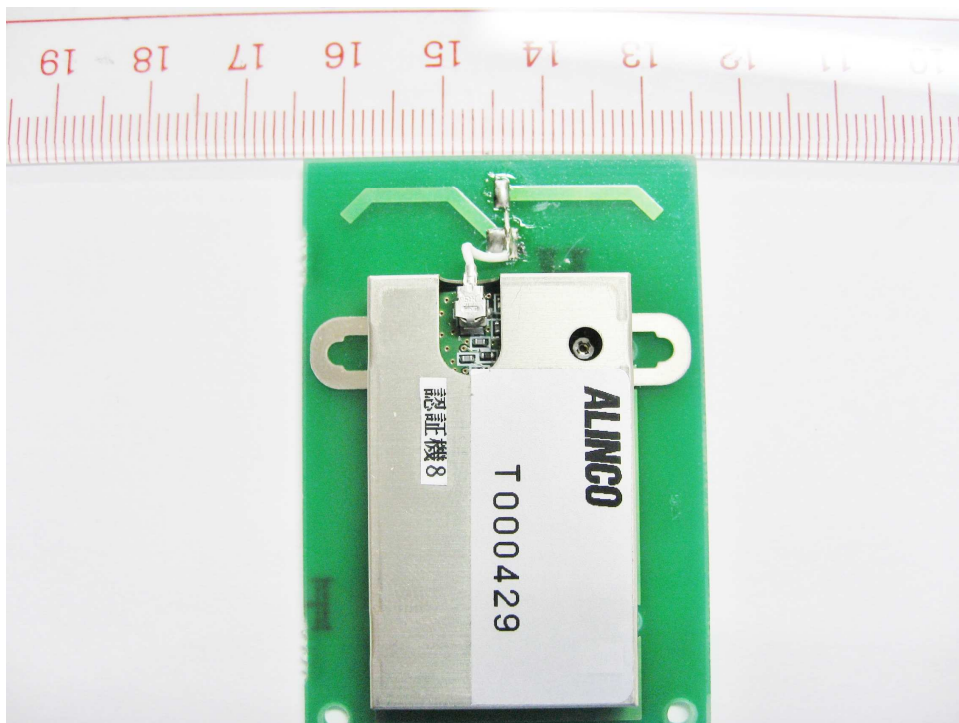
Antenna Type : Dipole Model No. 3148581510
