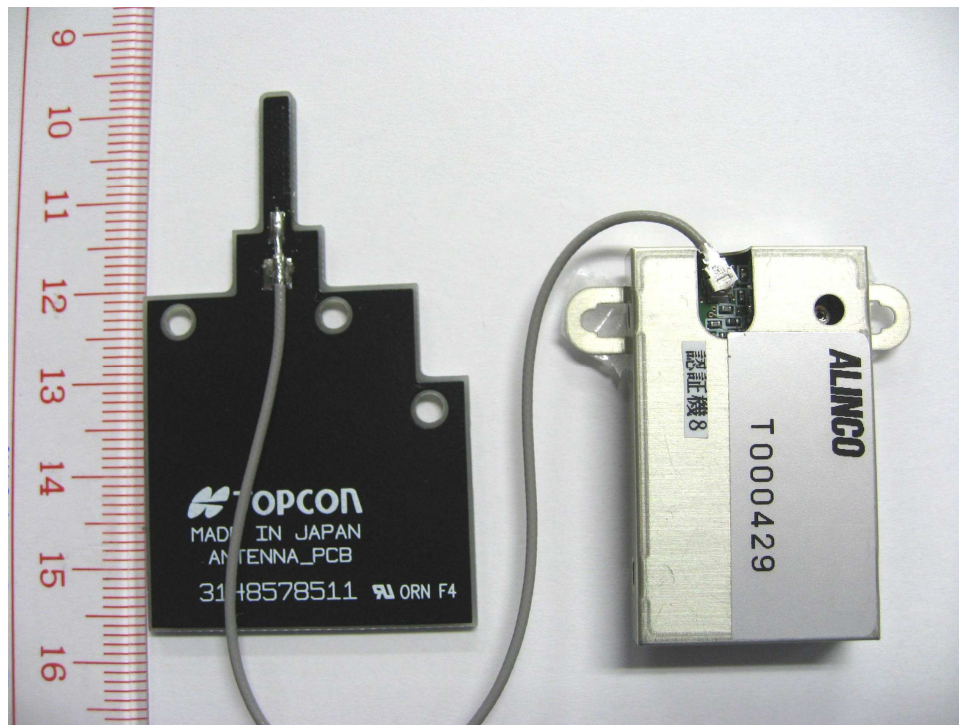
Antenna Type : Mono pole 1/4 Model No. 3148578511
