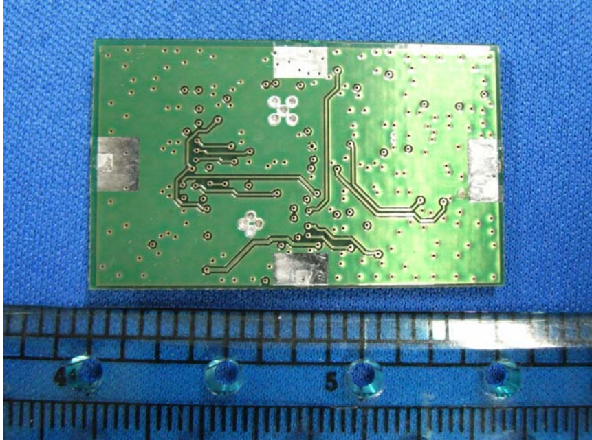
PCB Backside View
