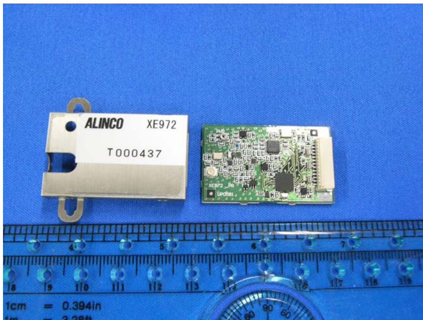
Top Case and inside PCB
