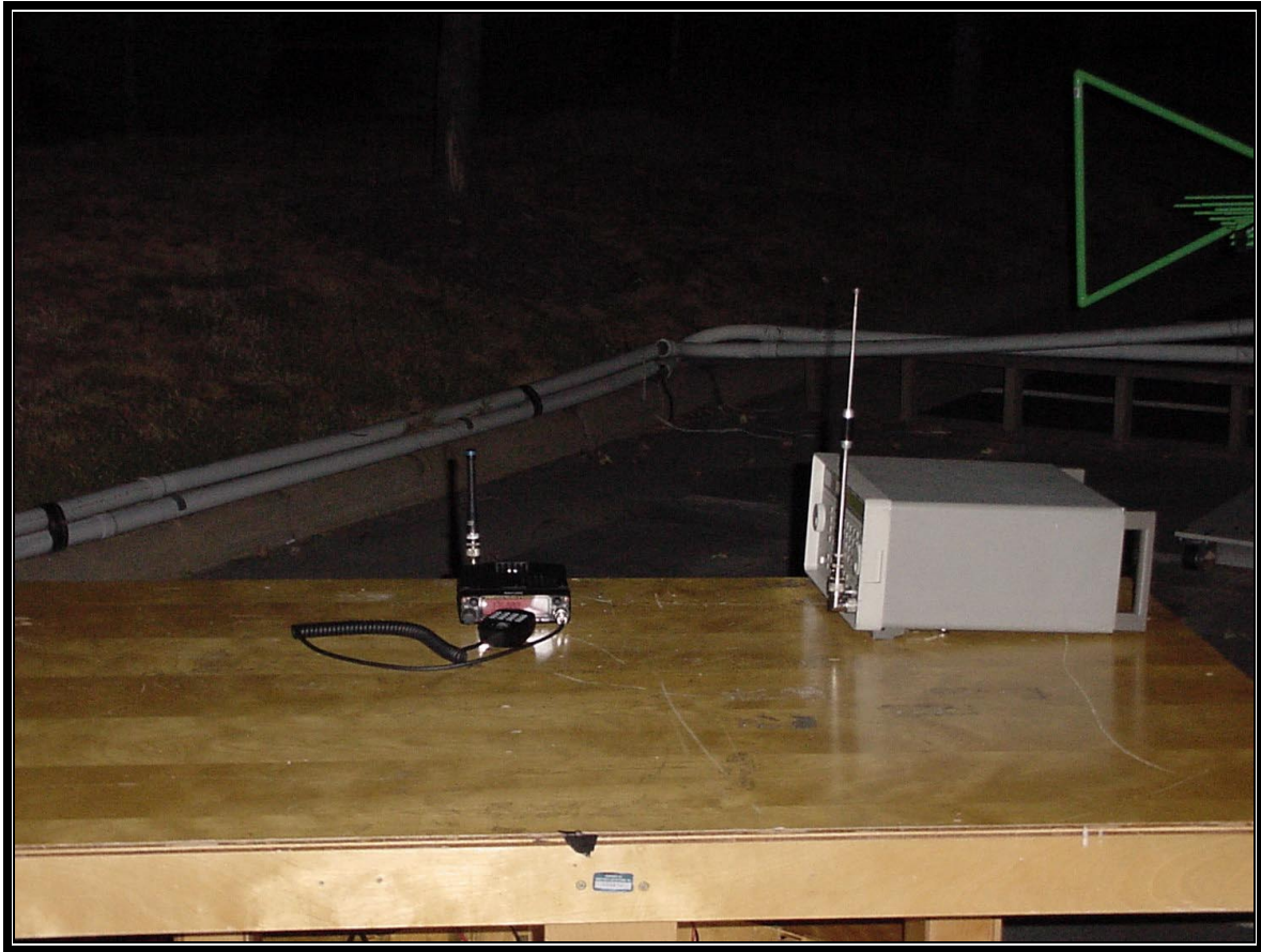
PHOTOGRAPH 4: RADIATED TEST CONFIGURATION (FRONT VIEW)
