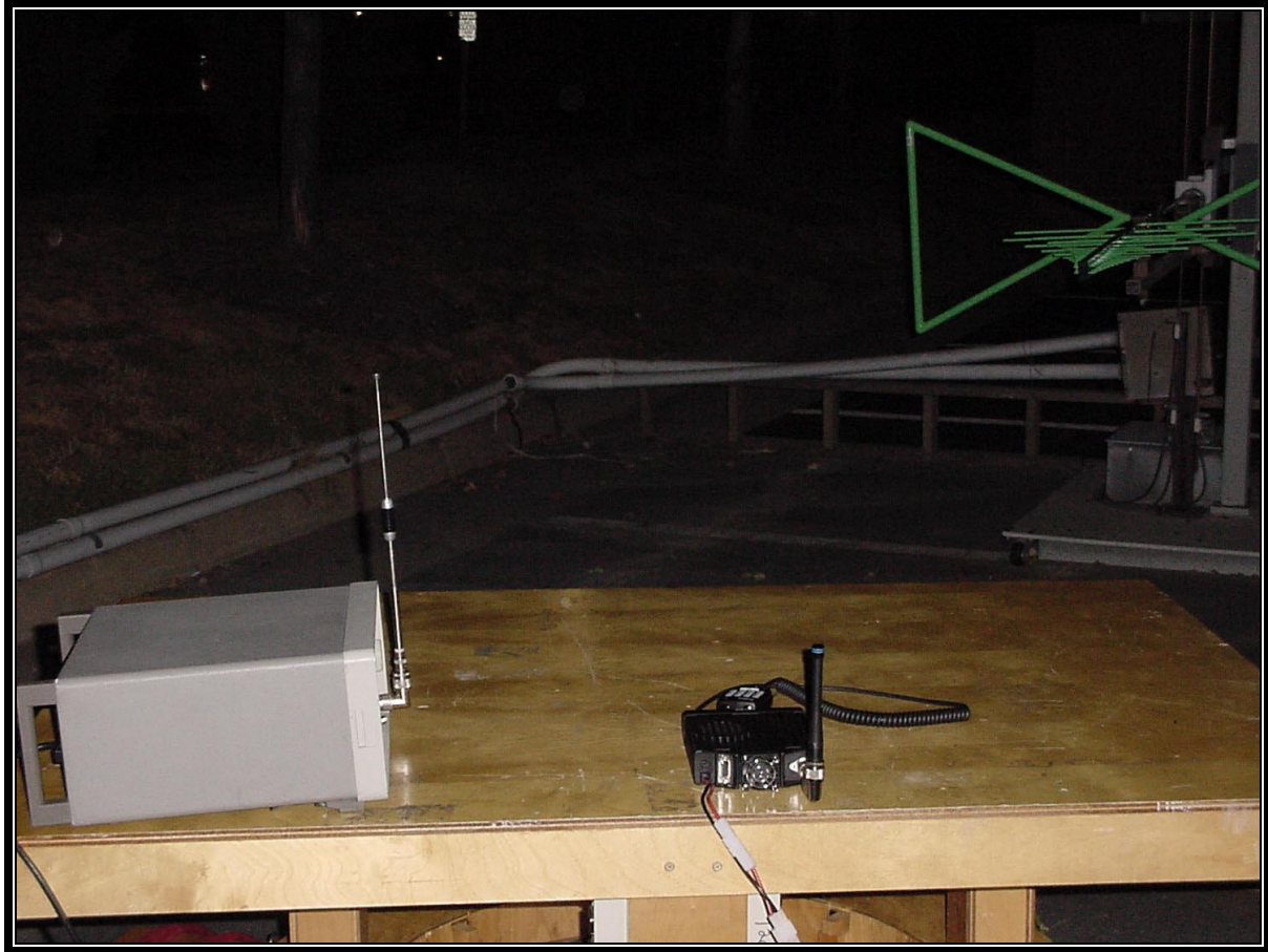
PHOTOGRAPH 5: RADIATED TEST CONFIGURATION (REAR VIEW)
