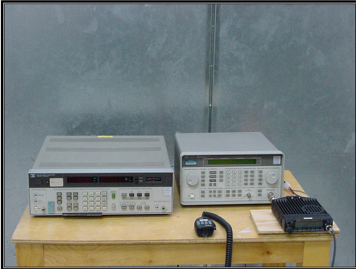
PHOTOGRAPH 6: 38DB SETUP
