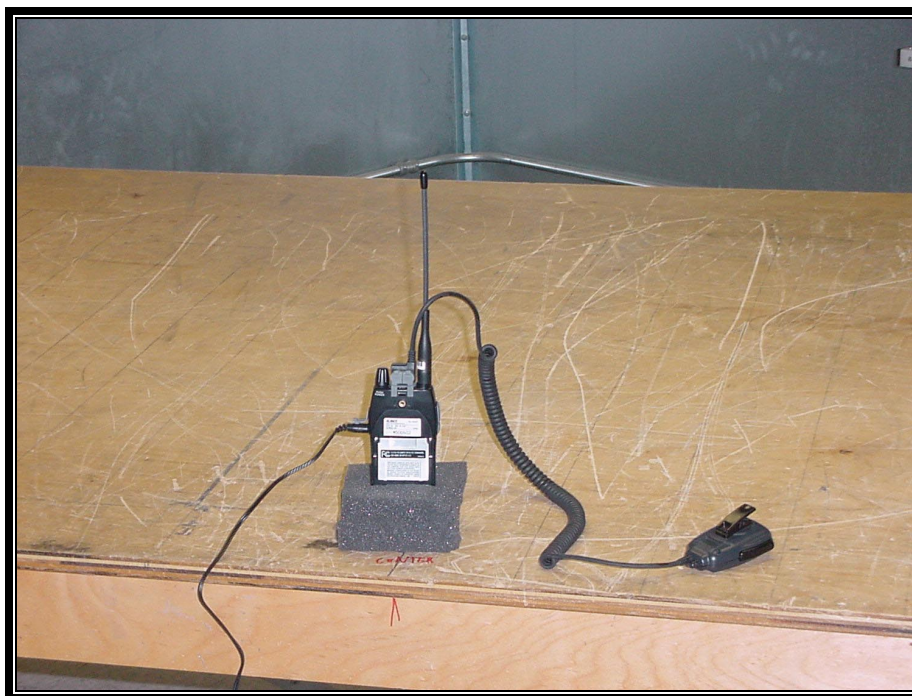
PHOTOGRAPH 2: CONDUCTED TEST CONFIGURATION (REAR VIEW)
