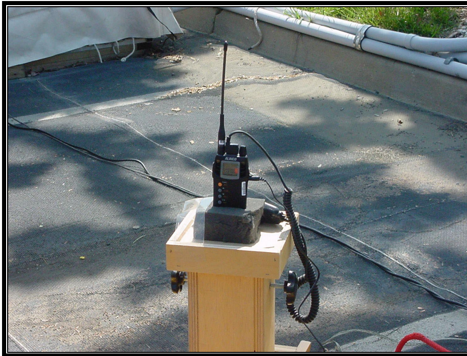
PHOTOGRAPH 3: RADIATED TEST CONFIGURATION (FRONT VIEW)
