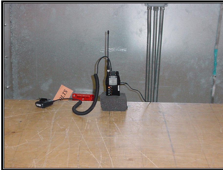
PHOTOGRAPH 1: CONDUCTED TEST CONFIGURATION (FRONT VIEW)
