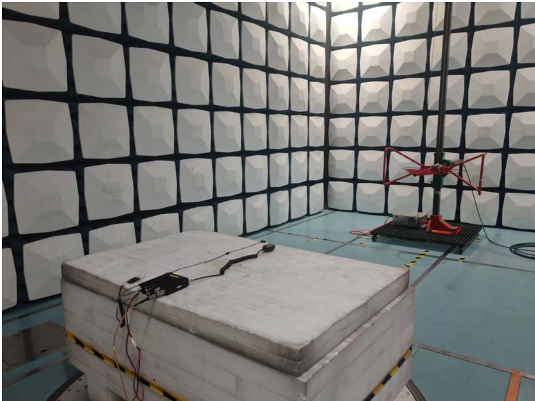
Radiated Emissions Below 1G side View M1-M2
