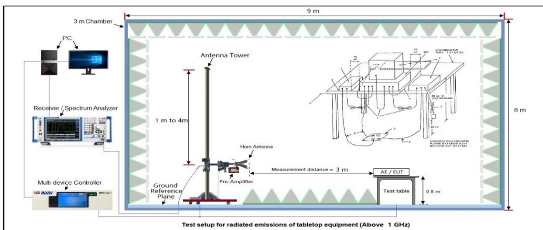
Radiated Emission Measurements Test Setup for above 1GHz
