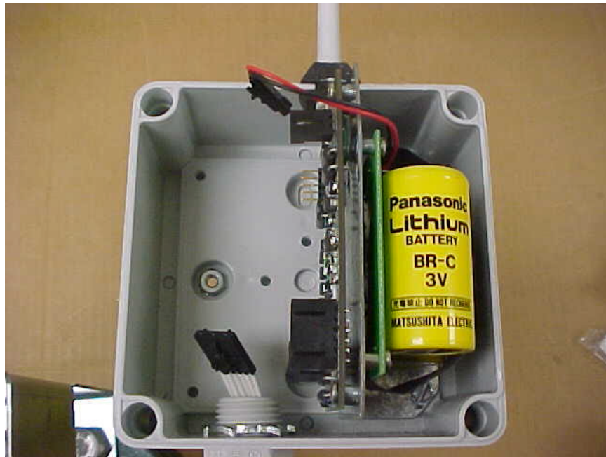
Close Look at the open cover for TANK UNIT
