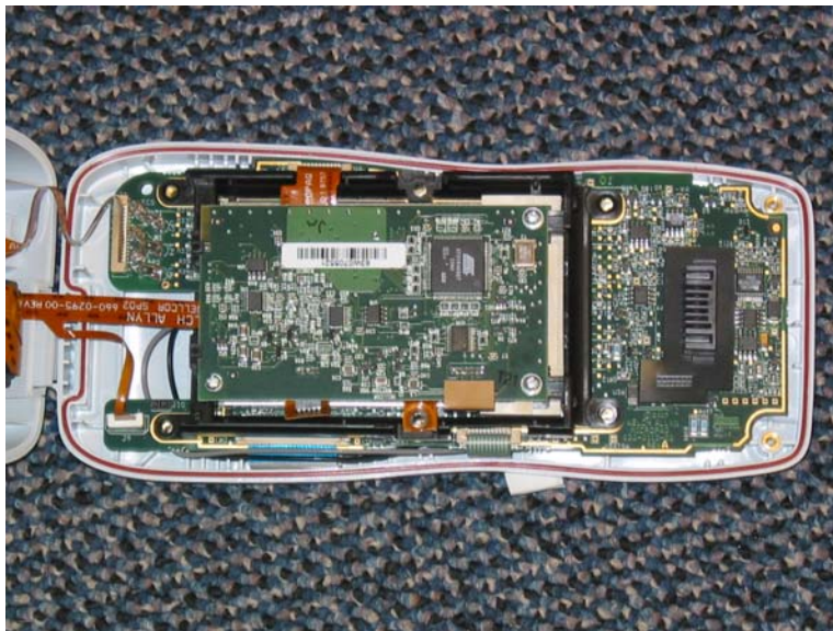
Back View of Unit with Cover Removed
