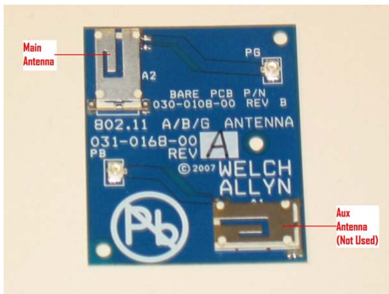
Front View of Antenna Board
