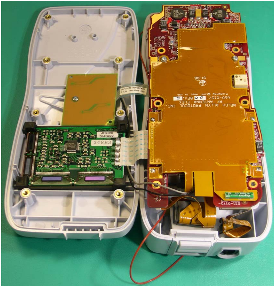
Internal Views End-Product
