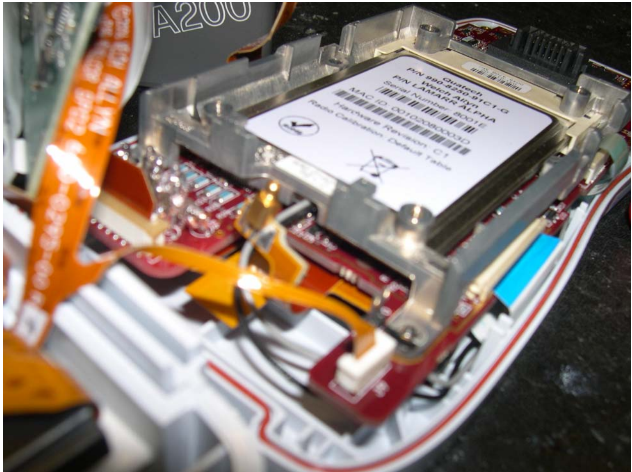
View of Radio Card Installed in End-Product
