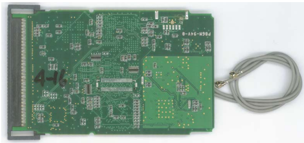
Bottom PCB View of PGUWA11A07
