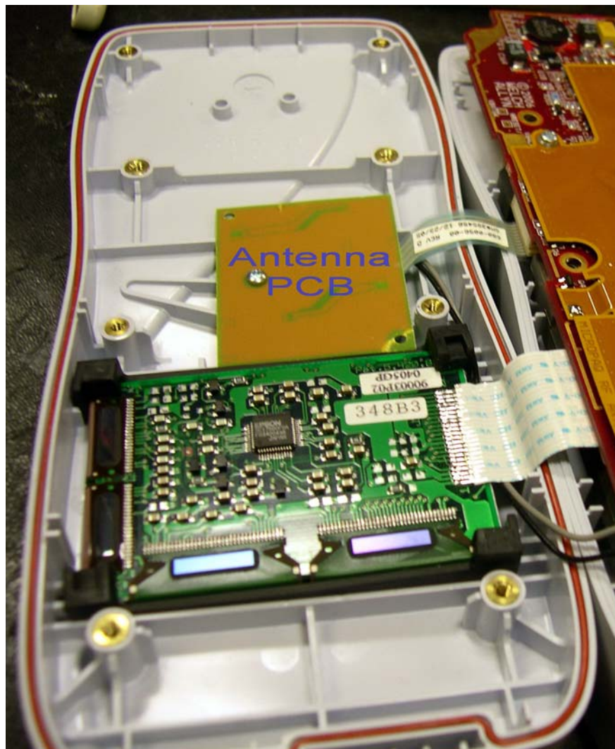
View of Antenna PCB Installed in End-Product
