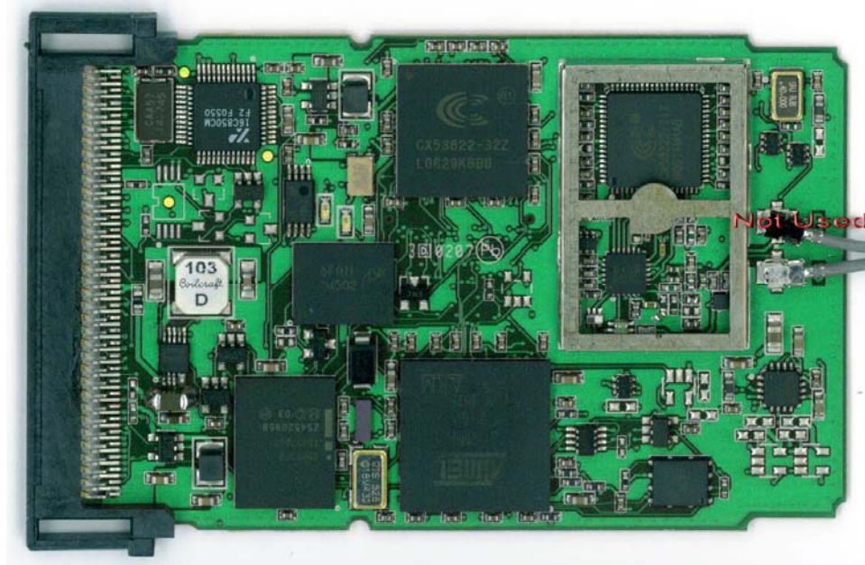
Top PCB View of PGUWA11A07 With EMI Shielding Cover Removed
