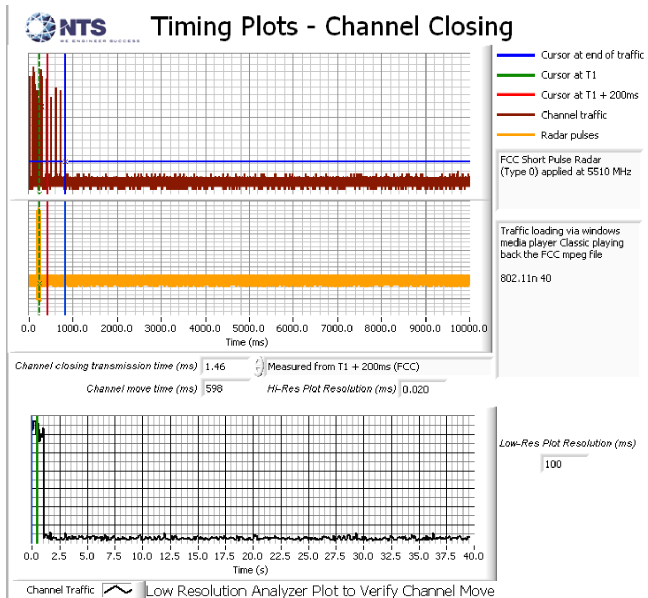
Figure 10 Channel Closing Time and Channel Move Time (n40 mode) – 40 second plot
