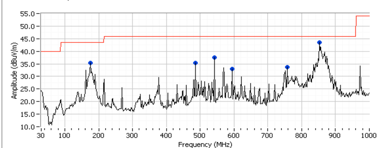
RF4CE at 2405 MHz; 802.11n 20MHz at 5825 MHz
