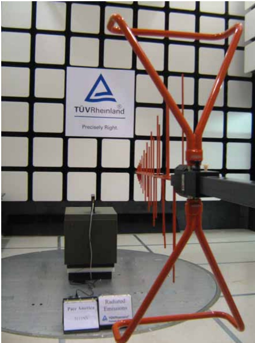
Figure 2: Test Setup for 30 MHz to 1000MHz (Rear View) – 5111NV on Vertical Position
