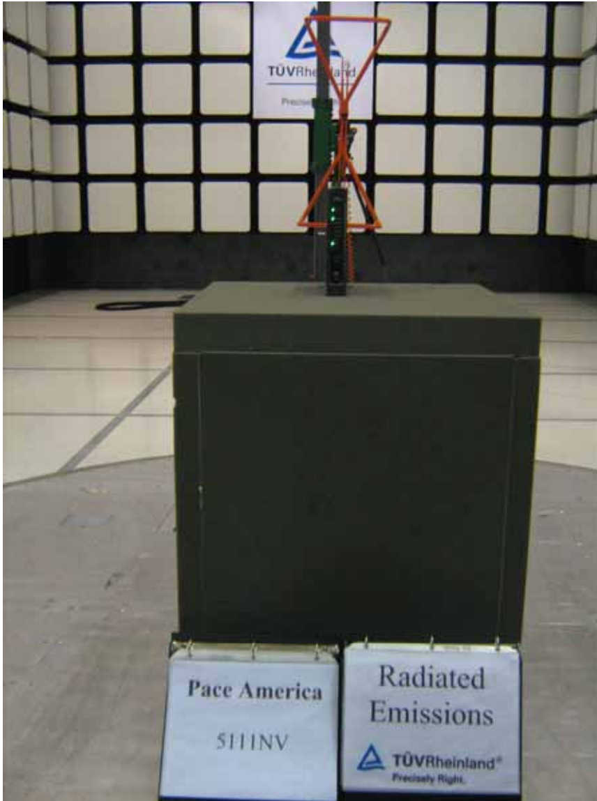
Figure 1: Test Setup for 30 MHz to 1000MHz (Front View) – 5111NV on Vertical Position
