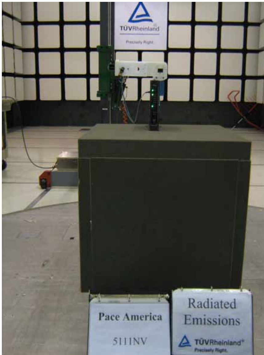
Figure 5: Test Setup for 18 GHz to 26GHz (Front View) – 5111NV on Vertical Position
