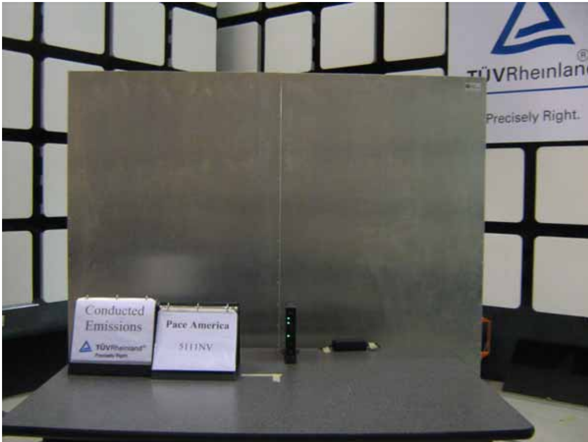
Figure 8: AC Conducted Emission Test Setup (Front View)
