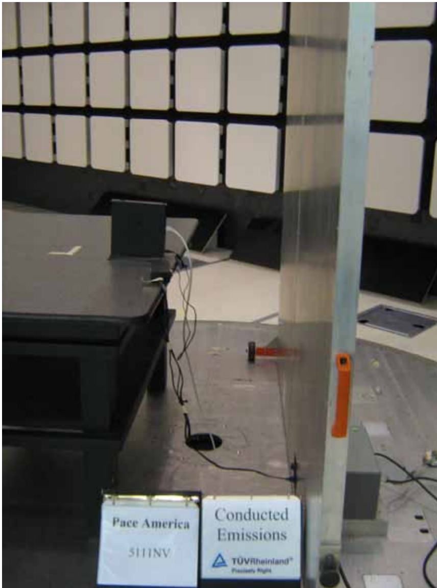
Figure 9: AC Conducted Emission Test Setup (Side View)
