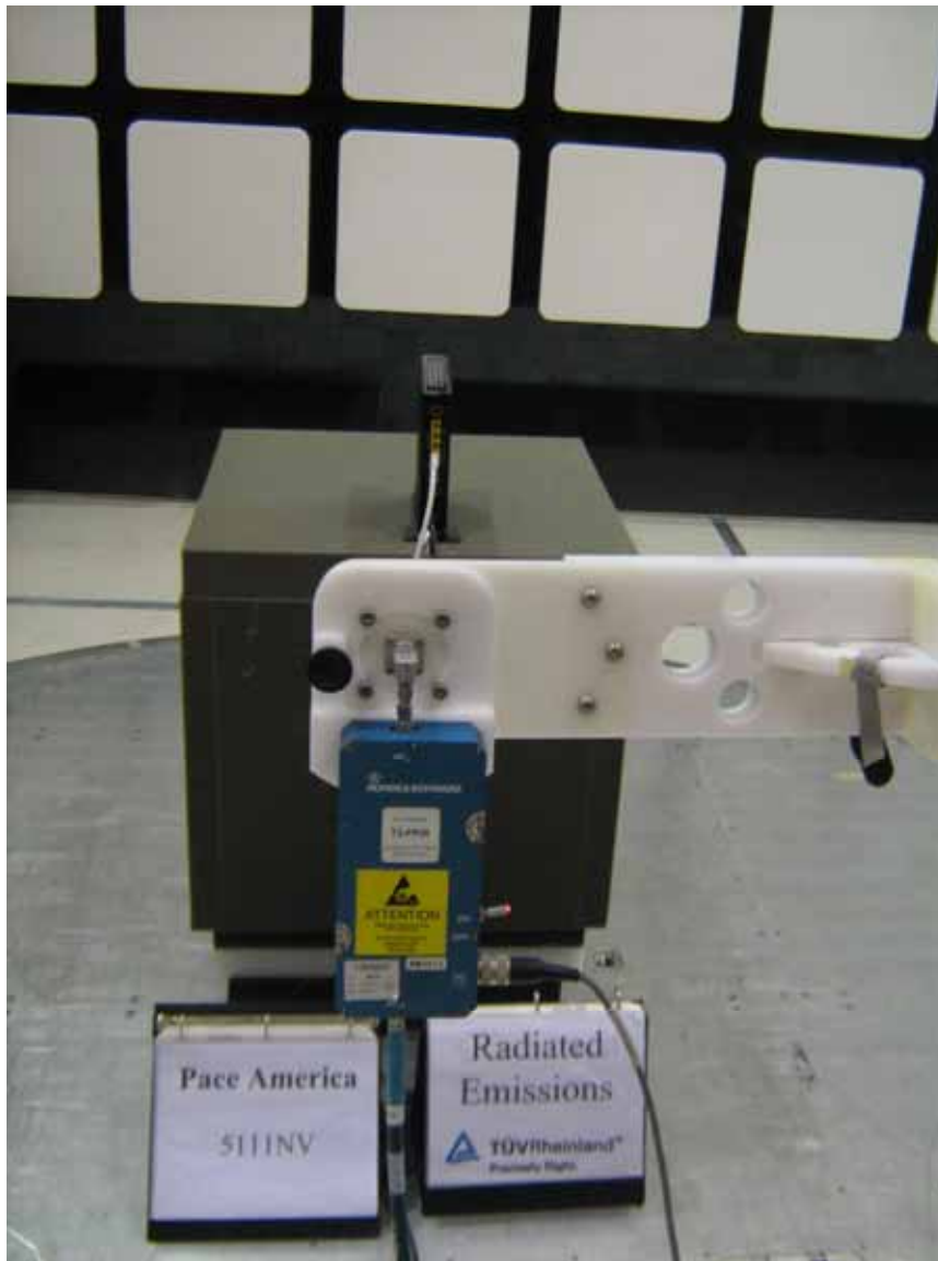
Figure 6: Test Setup for 18 GHz to 26GHz (Rear View) - 5111NV on Vertical Position
