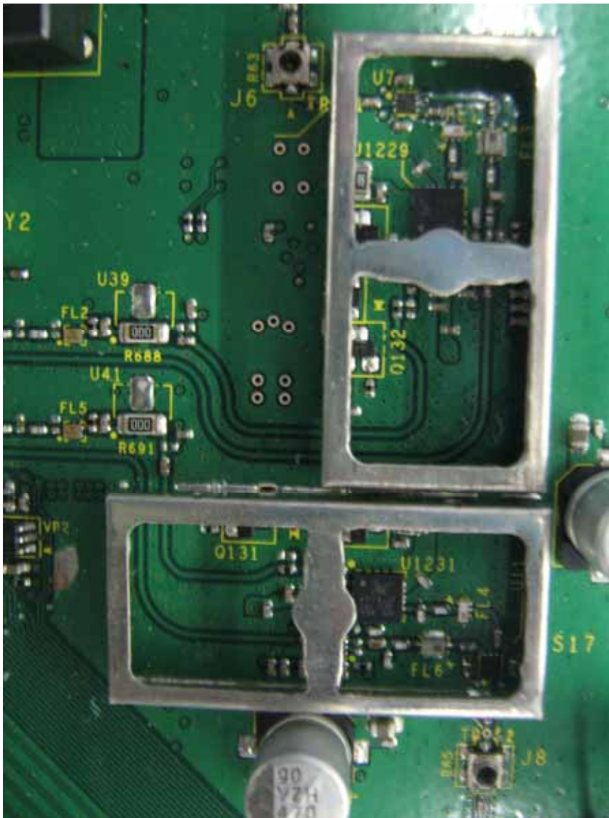
Figure 3: Internal Photo of 5111NV – Inside the Chipset RF Can
