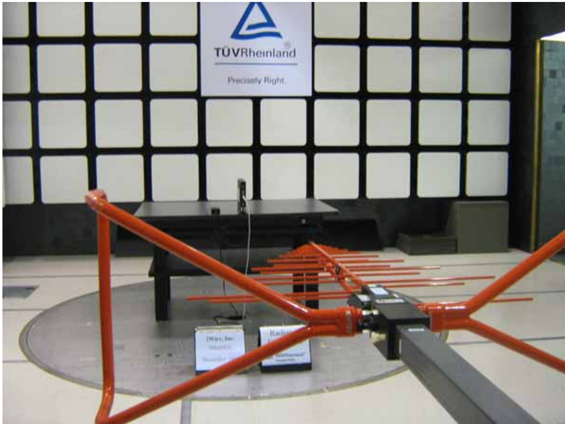
Figure 2: Test Setup for 30 MHz to 1000MHz (Rear View) – 3801HGV on Vertical Position
