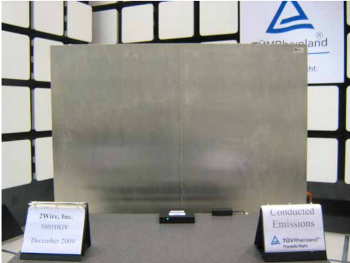
Figure 7: Photo of Test Setup for HomePortal 3801HGV, AC Conducted Emission (Front View)
