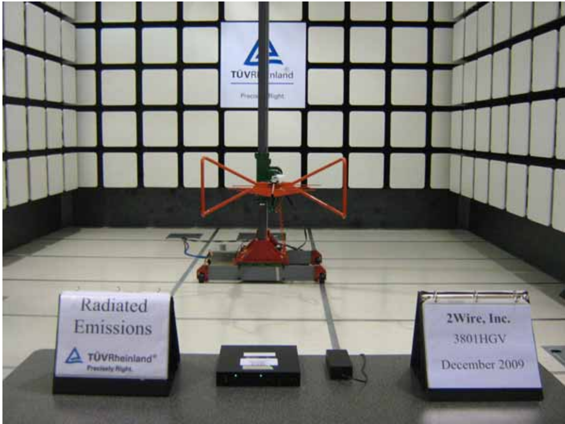
Figure 1: Test Setup for 30 MHz to 1000MHz (Front View) – 3801HGV on Horizontal Position
