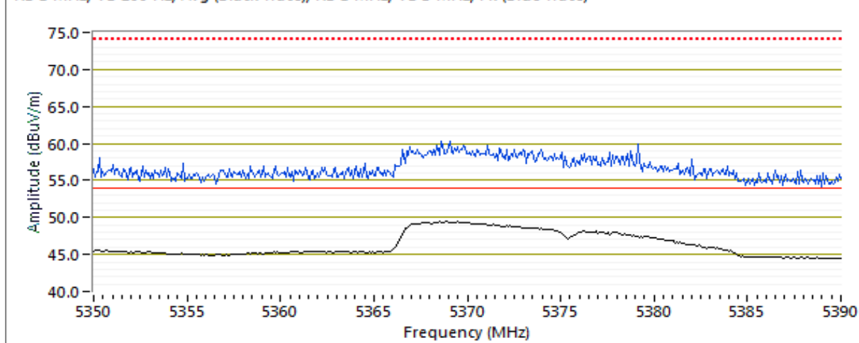
RB 1 MHz; VB 200 Hz; Avg (Black Trace); RB 1 MHz; VB 3 MHz; Pk (Blue Trace)
