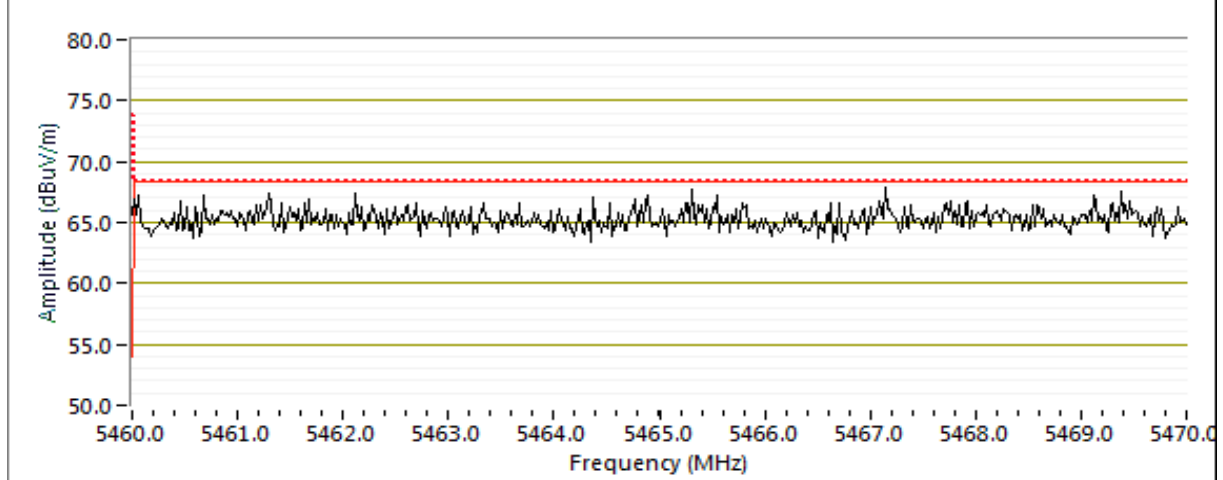
RB 1 MHz; VB 3 MHz; Pk (Black Trace)
