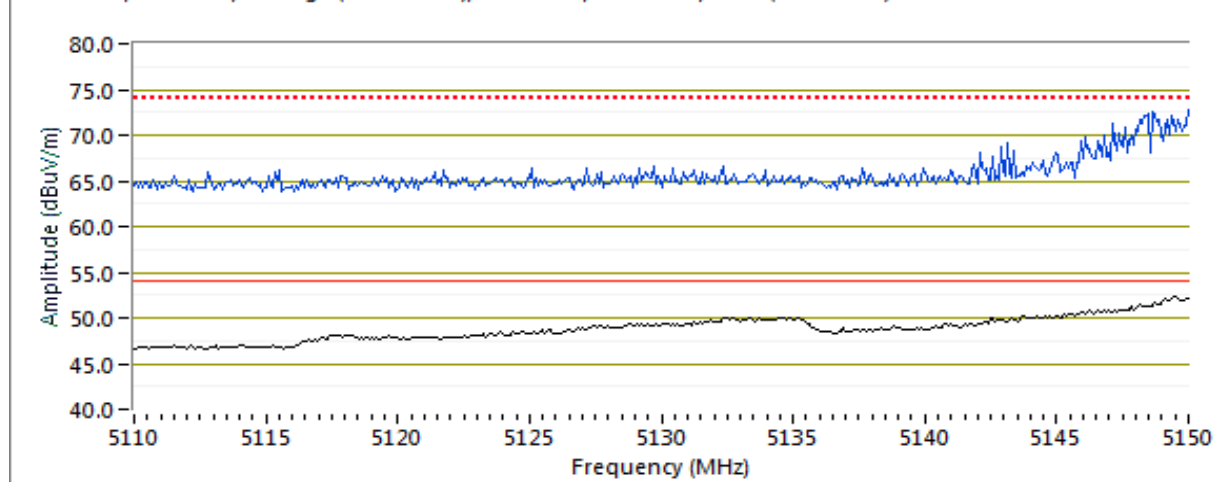
RB 1 MHz; VB 1 kHz; Average (Black Trace); RB 1 MHz; VB 3 MHz; Peak (Blue Trace)
