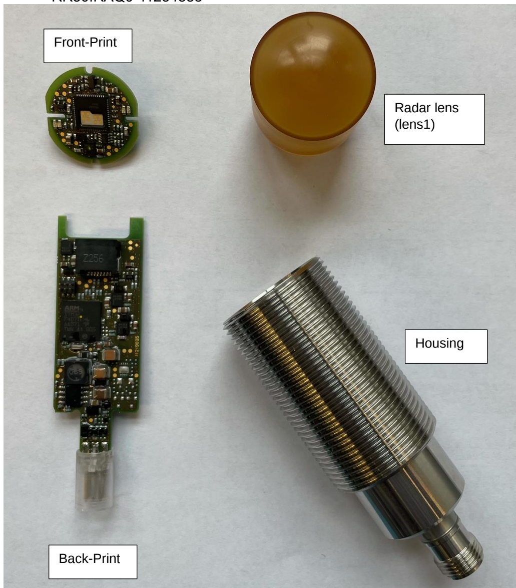
Main components of a RR30 radar sensor (lens type 1)
