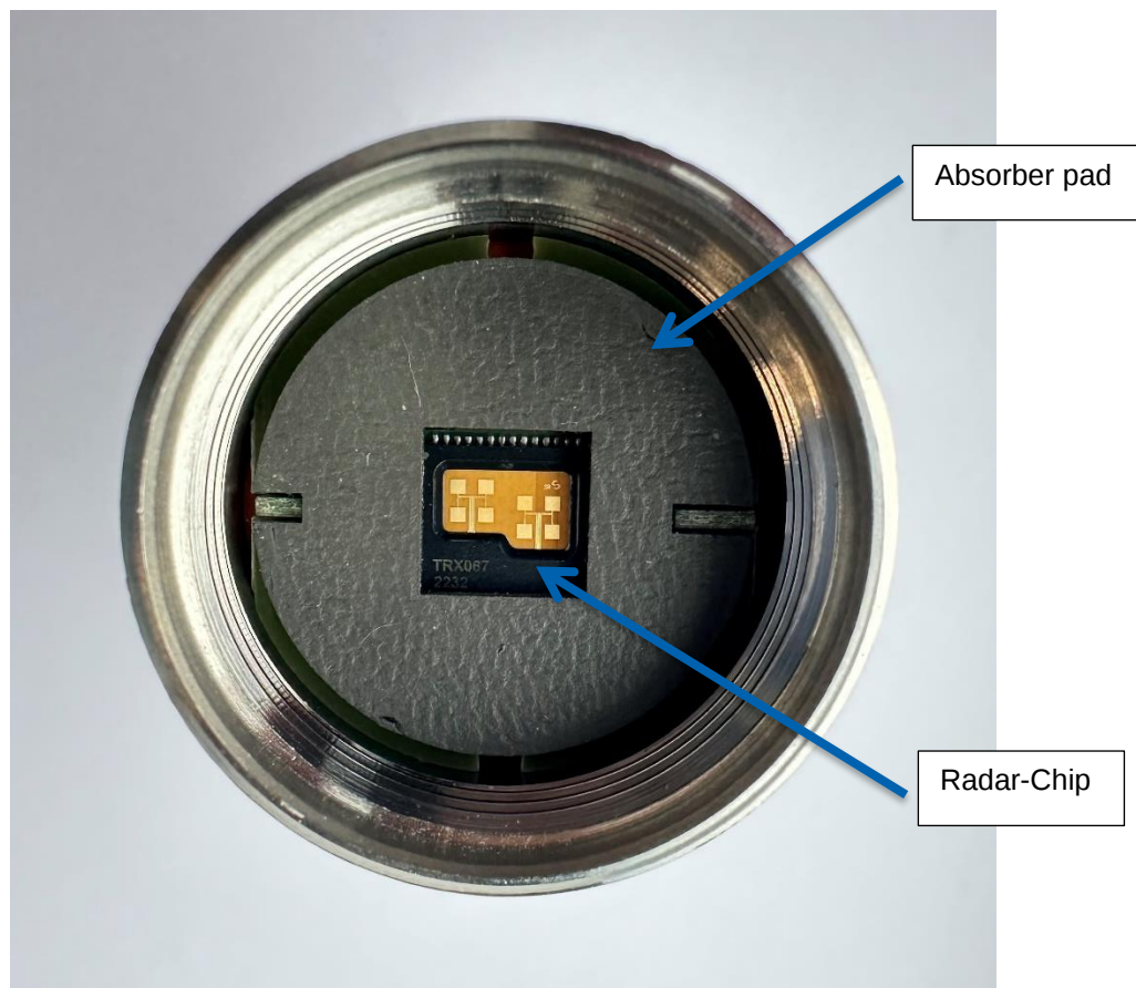
Back-Print and Front-Print inside housing with absorber pad
