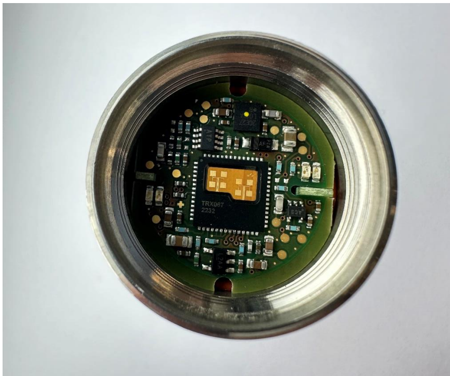
Back-Print and Front-Print inside housing
