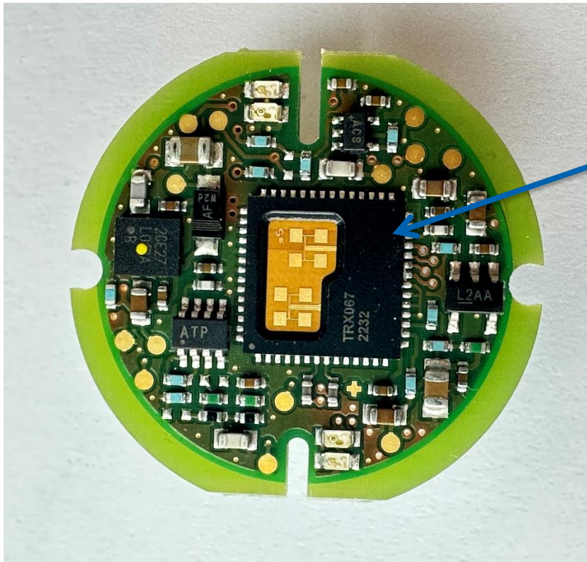
Front-Print: Top-View
