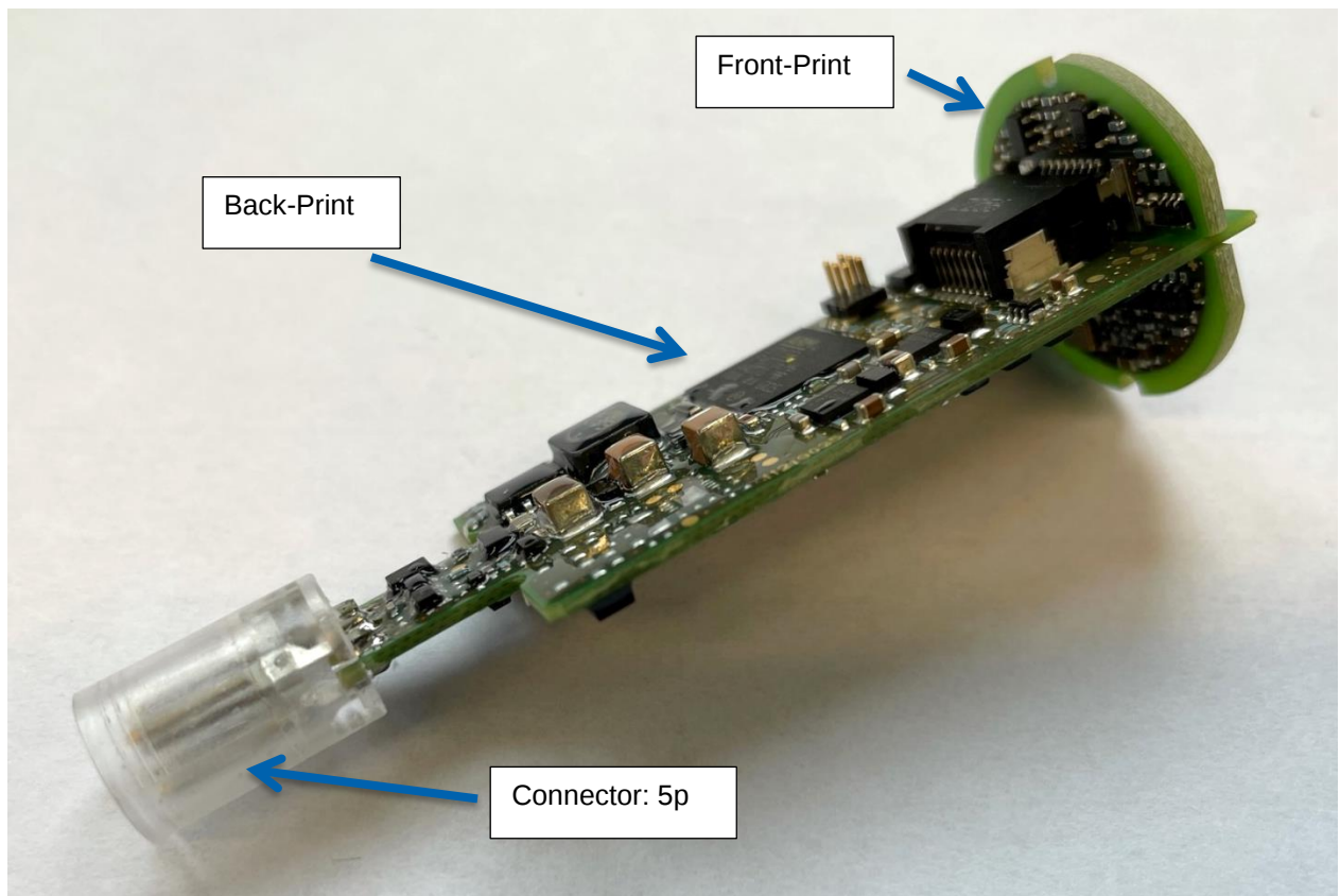
Back-Print and Front-Print connected
