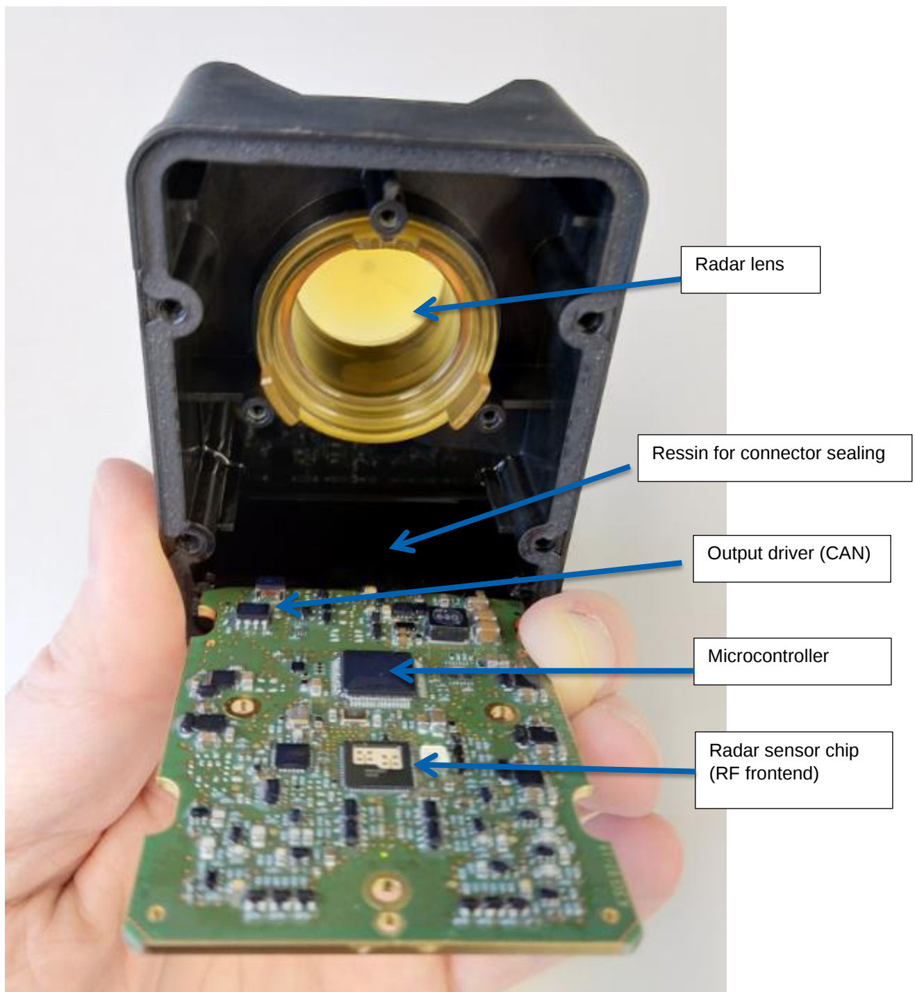
R600V Sensor with PCBA folded out
