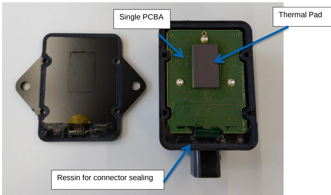
R600V Sensor with removed back cover
