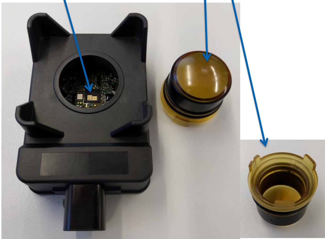
Rader sensor with removed lens → direct view to the radar chip (RF frontend)
