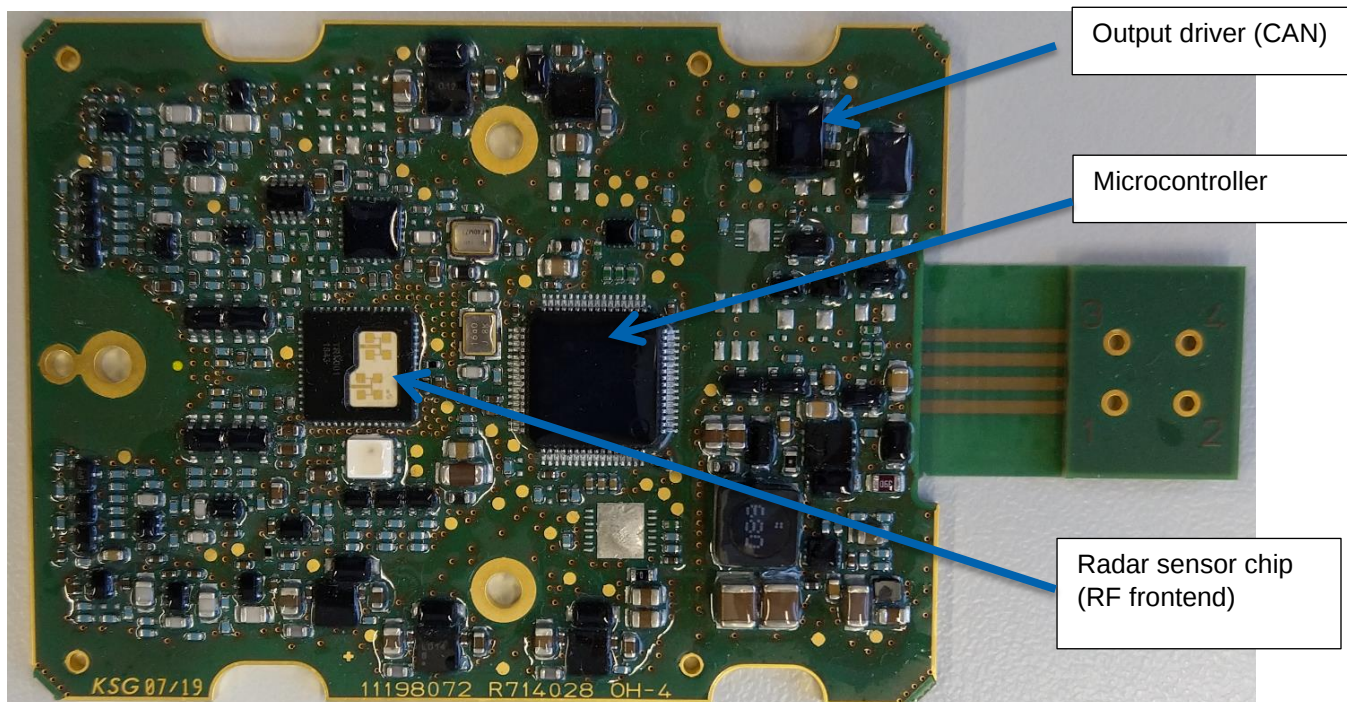
Top-View of PCBA
