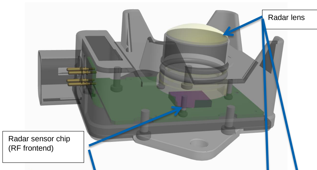
Radar sensor as a model
