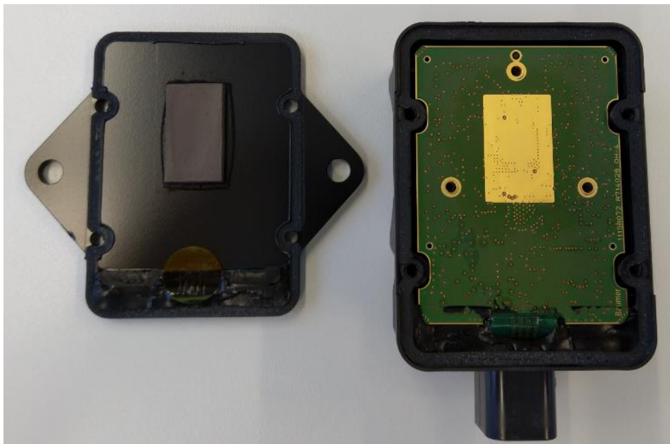
R600V Sensor with removed back cover
