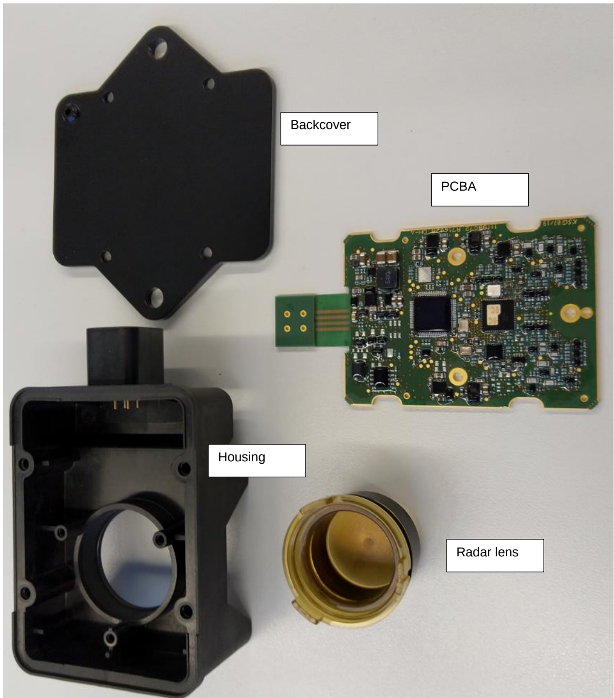
Main components of a R600V radar sensor
