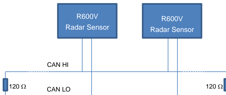
Fig 8 CAN connection setup diagram
