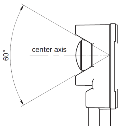
Fig 6 Recommended Free Space
