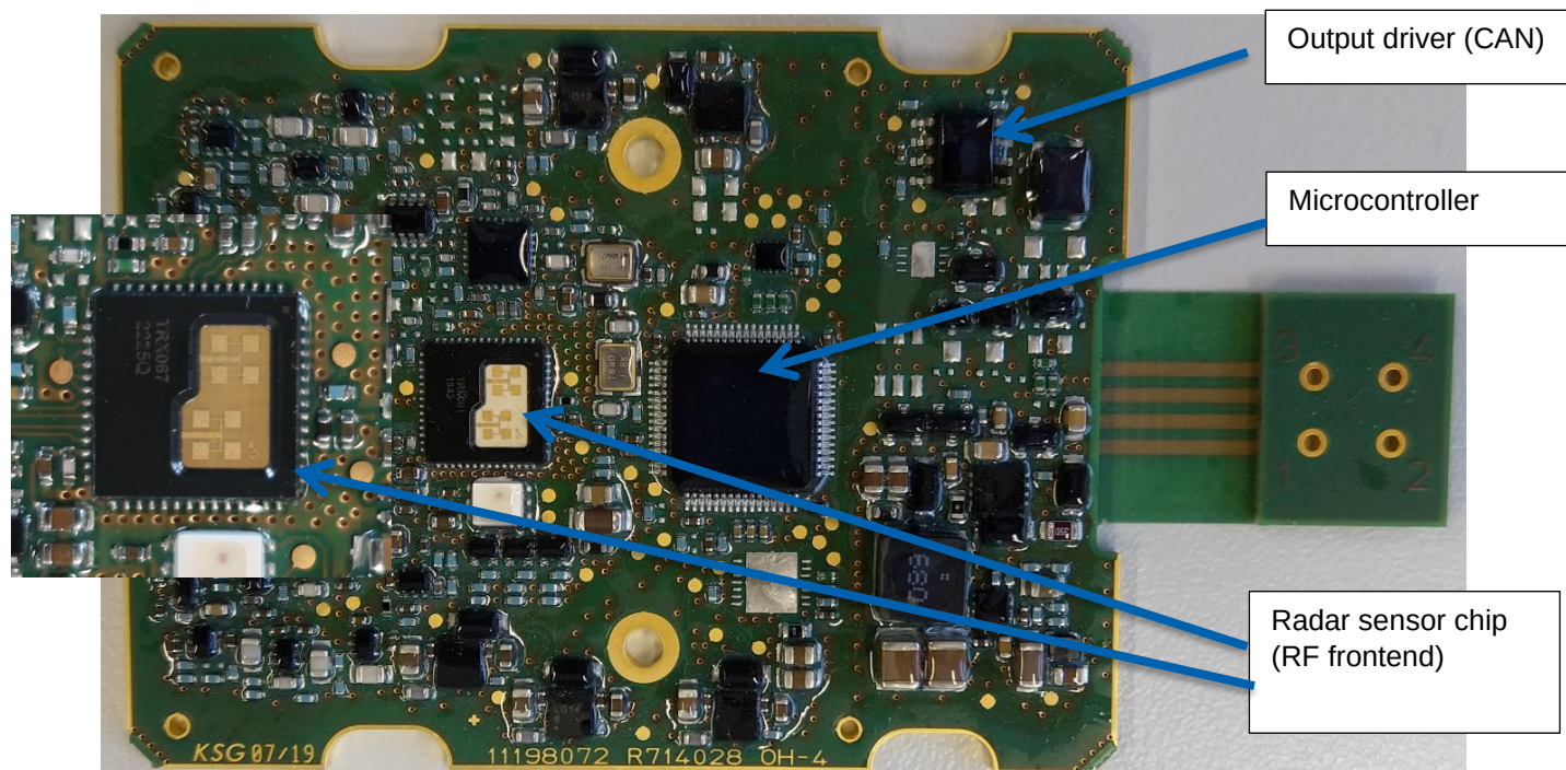
Top-View of PCBA
